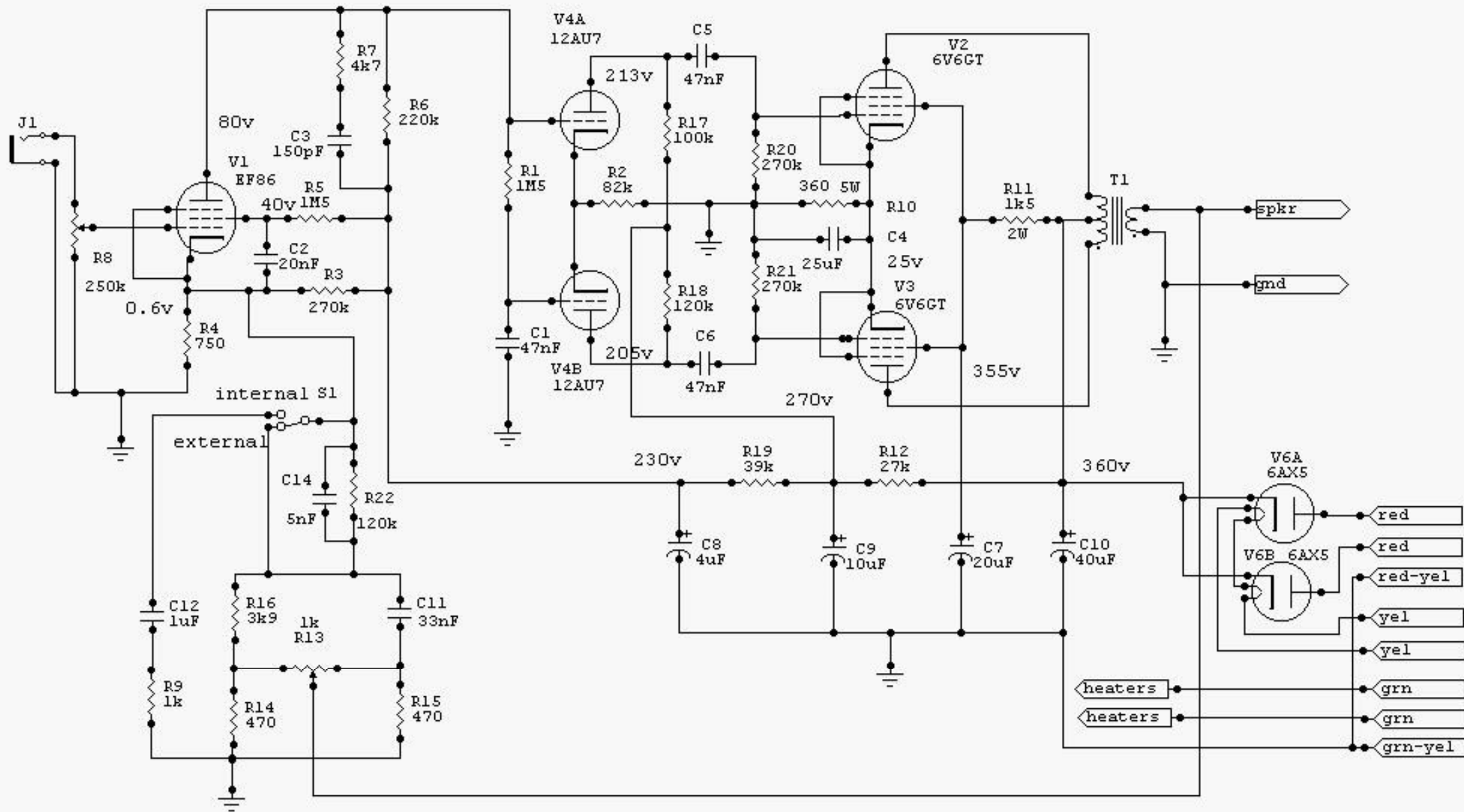
Ampex 612 Speaker Amplifier Drawn: 1/21/2000
