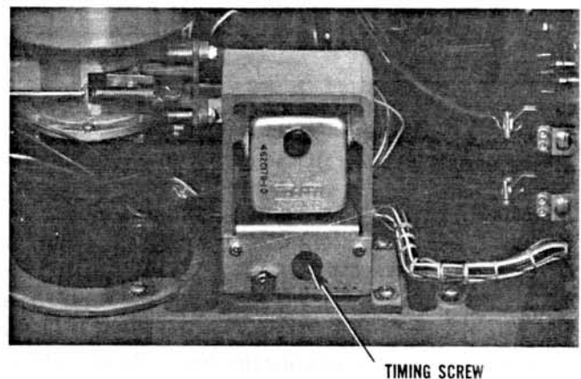
Fig. 4-3. Timing Adjustment--Transducer
