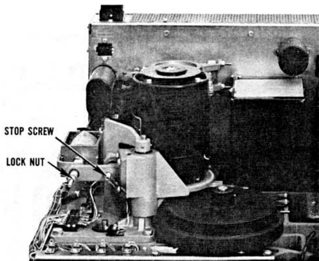
Fig. 4-5. Tape Speed Adjustment
