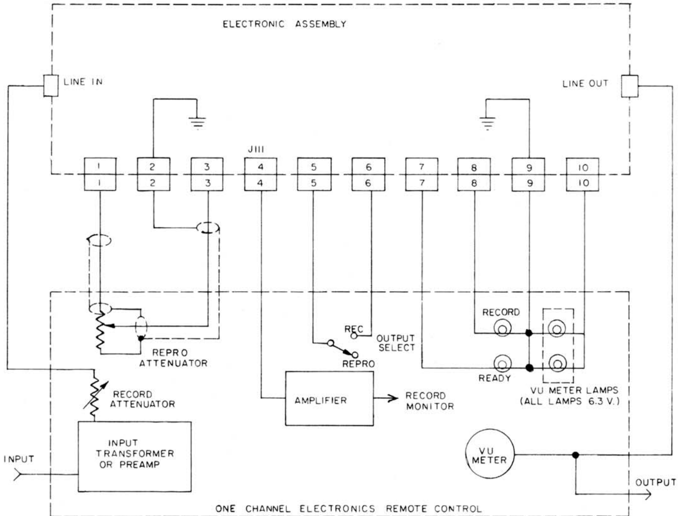
Fig. 2-2. Suggested Electronic Remote Control
