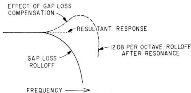
Fig. 5-7. Head Gap Compensation
