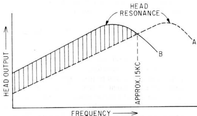
Fig. 5-5 Result of Moving Head Resonance
