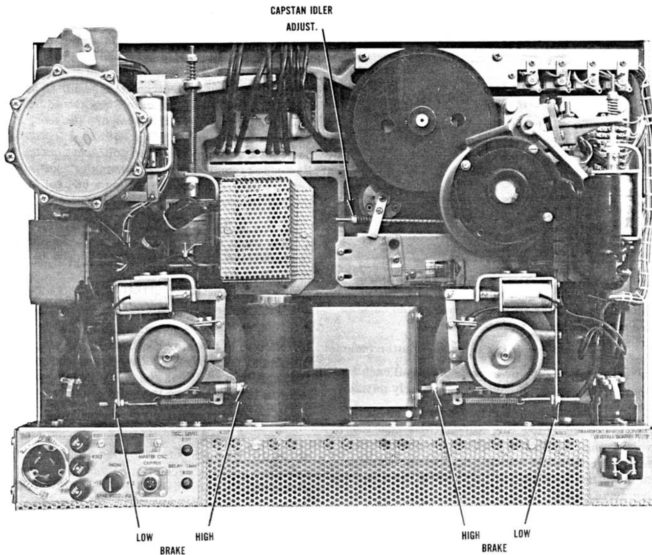
Fig. 4-4. Brake and Idler Adjustment
