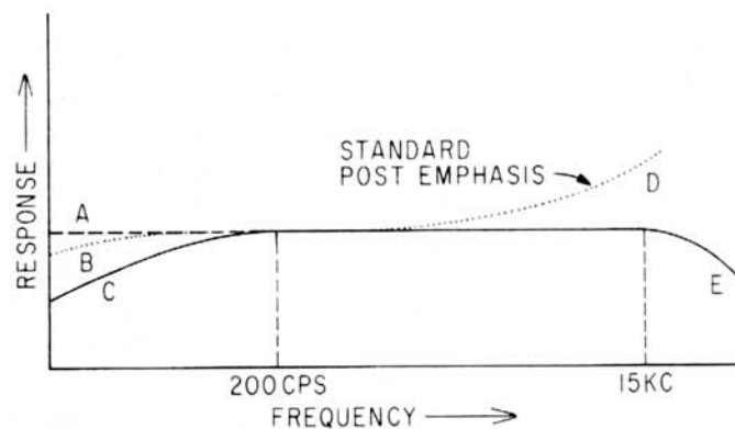
Fig. 5-6. Final Response
