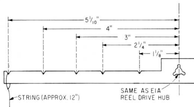
Fig. 4-1. Special Tool for Checkout
