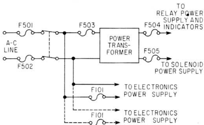
Fig. 4-6. Fusing Diagram
