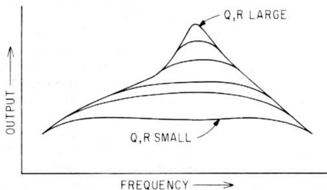
Fig. 5-4. Flattening Head Output
