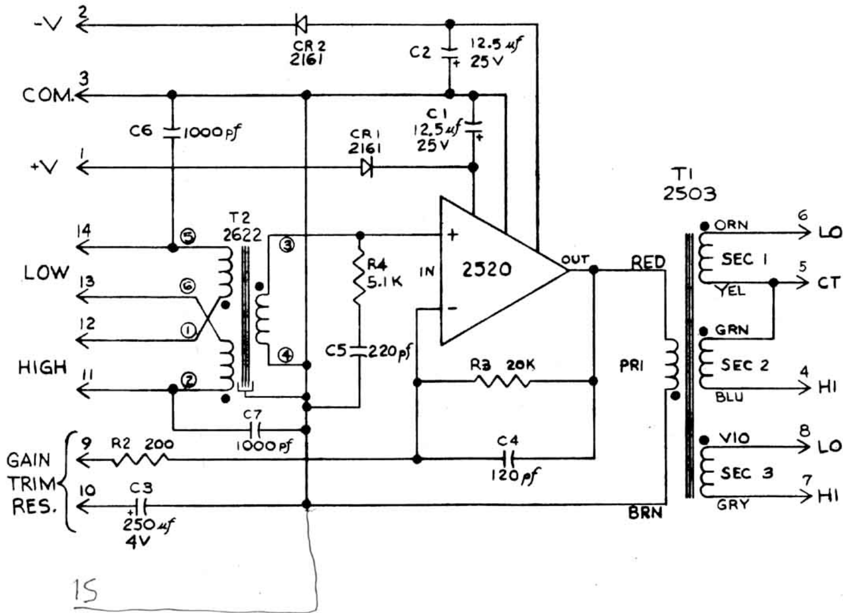
MIC PREAMP SCHEMATIC
