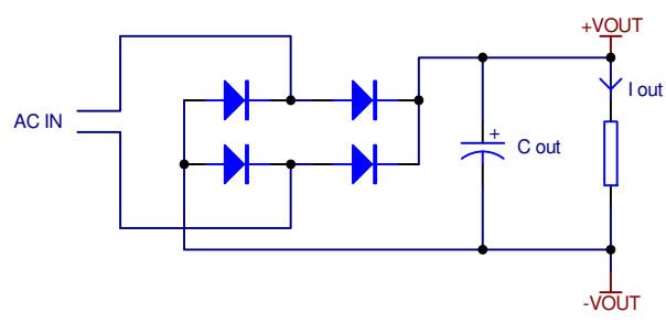
TEST CIRCUIT (PER OUTPUT)
