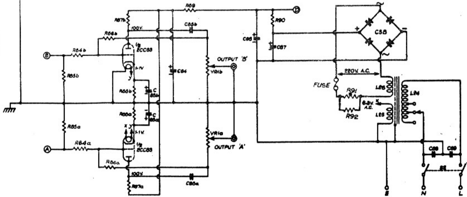
CIRCUIT DIAGRAM OF MODEL 223
