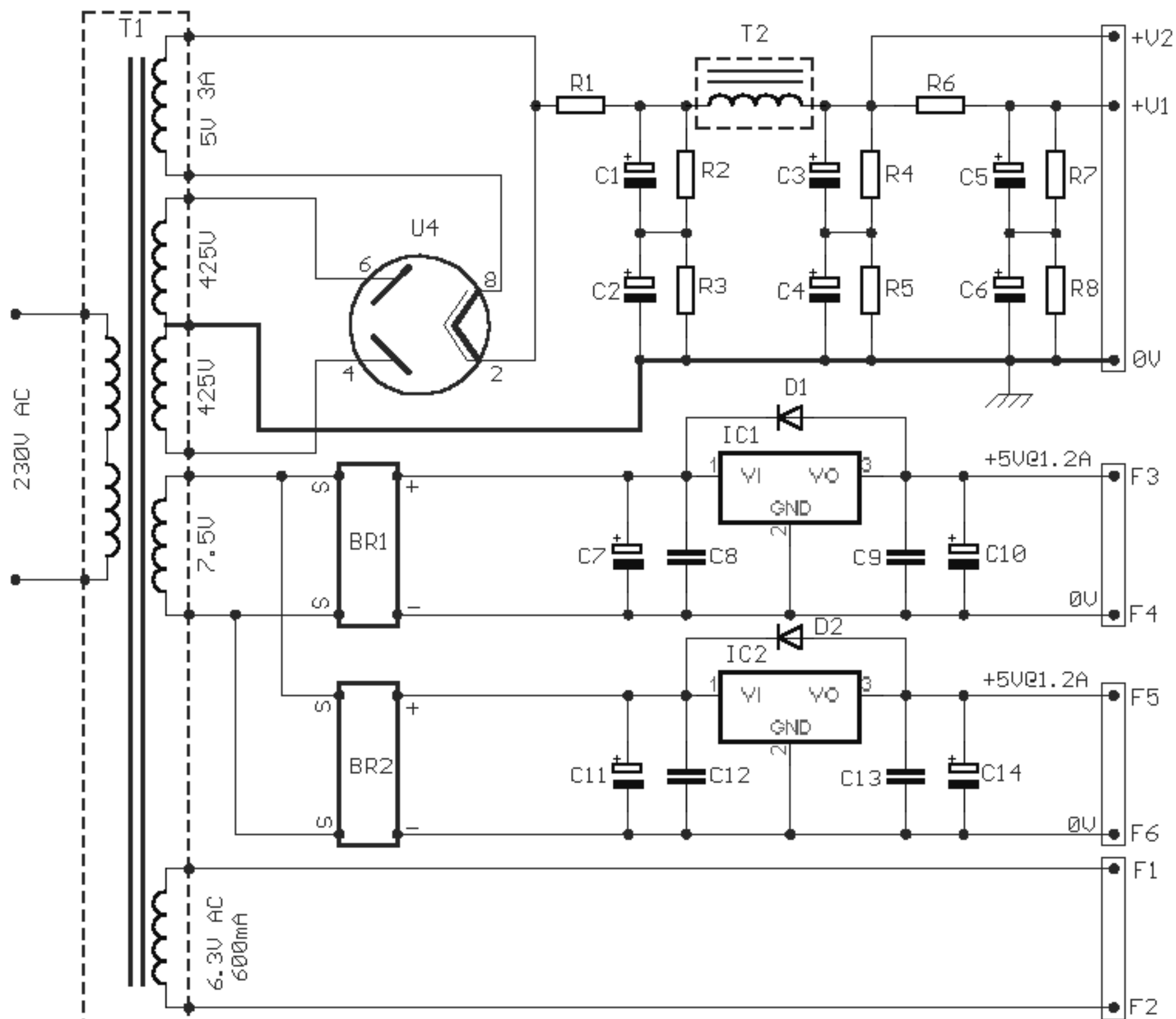
Fig.2- POWER SUPPLY FOR AUDIO NOTE CONQUEST
