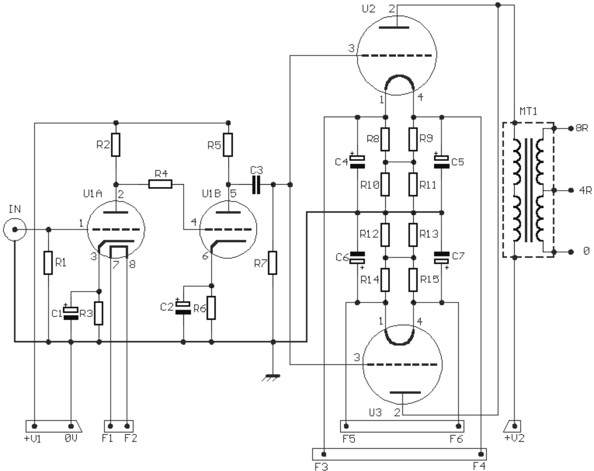
Fig.1- AUDIO NOTE CONQUEST 300B POWER AMPLIFIER Sam 3/02
