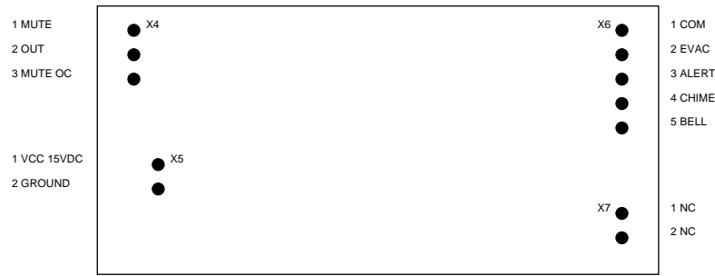
AM Tone Module PCB 6360 (Top View)
