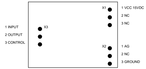
AM VCA CONTROL MODULE PCB 6364 (TOP VIEW)
