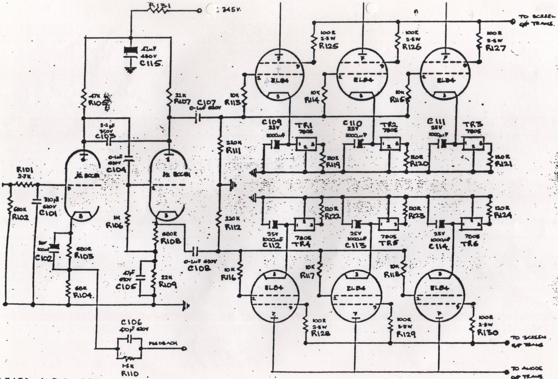
BEARD AUDIO P.35 ONE CHANNEL
