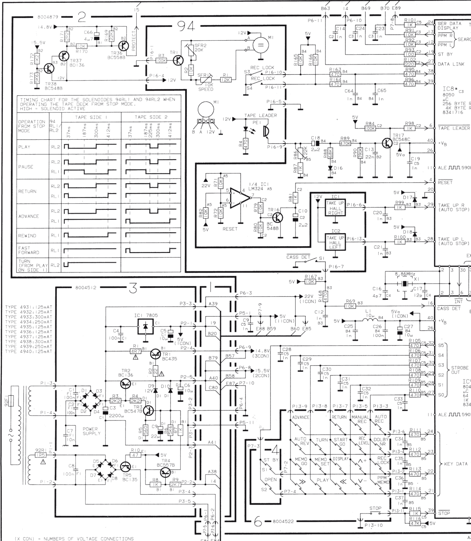
DIAGRAM D, TAPE DECK VERSION II, (Control Circuits, Power Supply)
