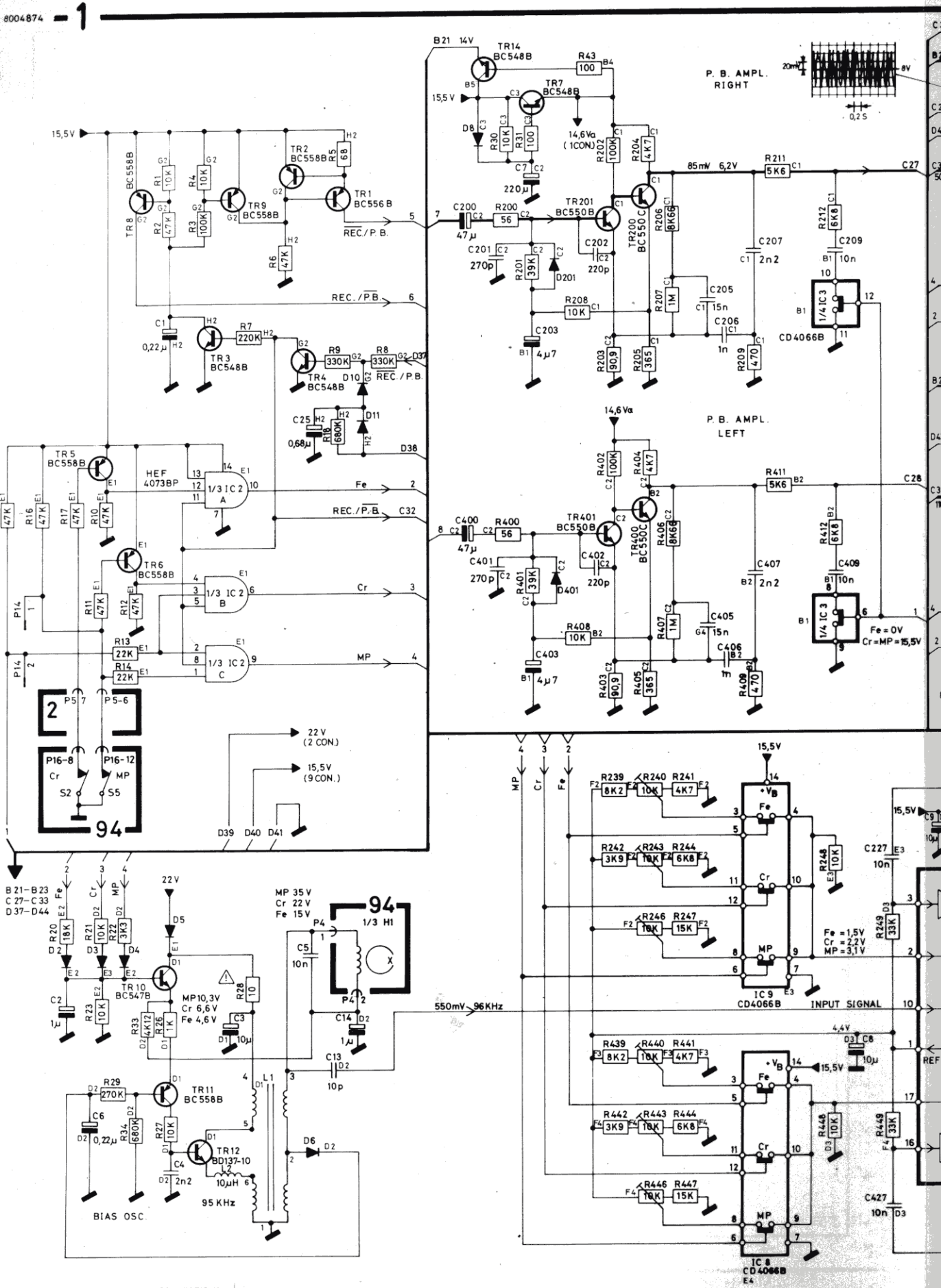
DIAGRAM A, TAPE DECK VERSION II, (Bais Osc, P.B. Ampl., Rec. Ampl., HX PRO)
