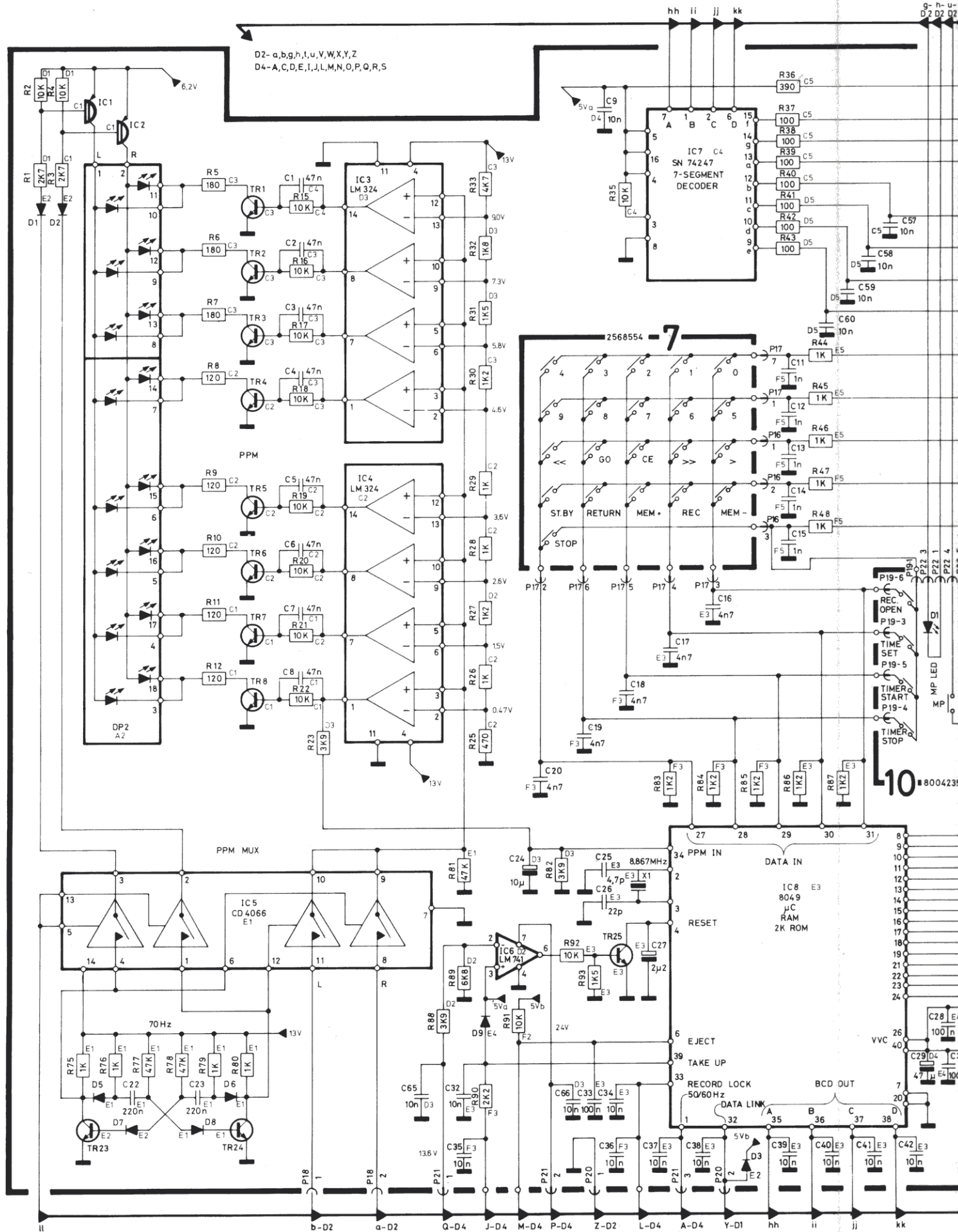
DIAGRAM 3 FOR BEOCORD 8002
