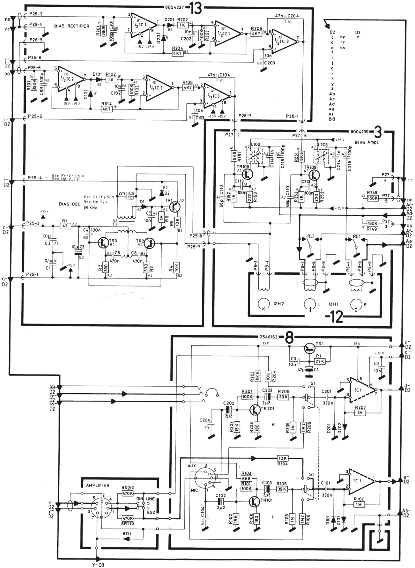
DIAGRAM 1 FOR BECORD 8002
