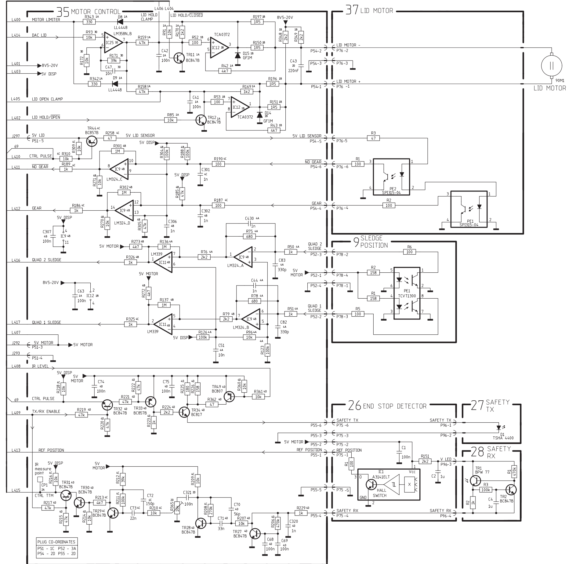
DIAGRAM M – Motor Control and Detection
