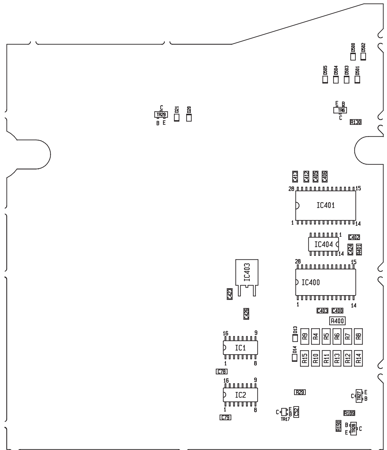
PCB32, Input/output Select, Sound Adjustment – secondary side
