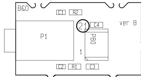
PCB21, Headphone
