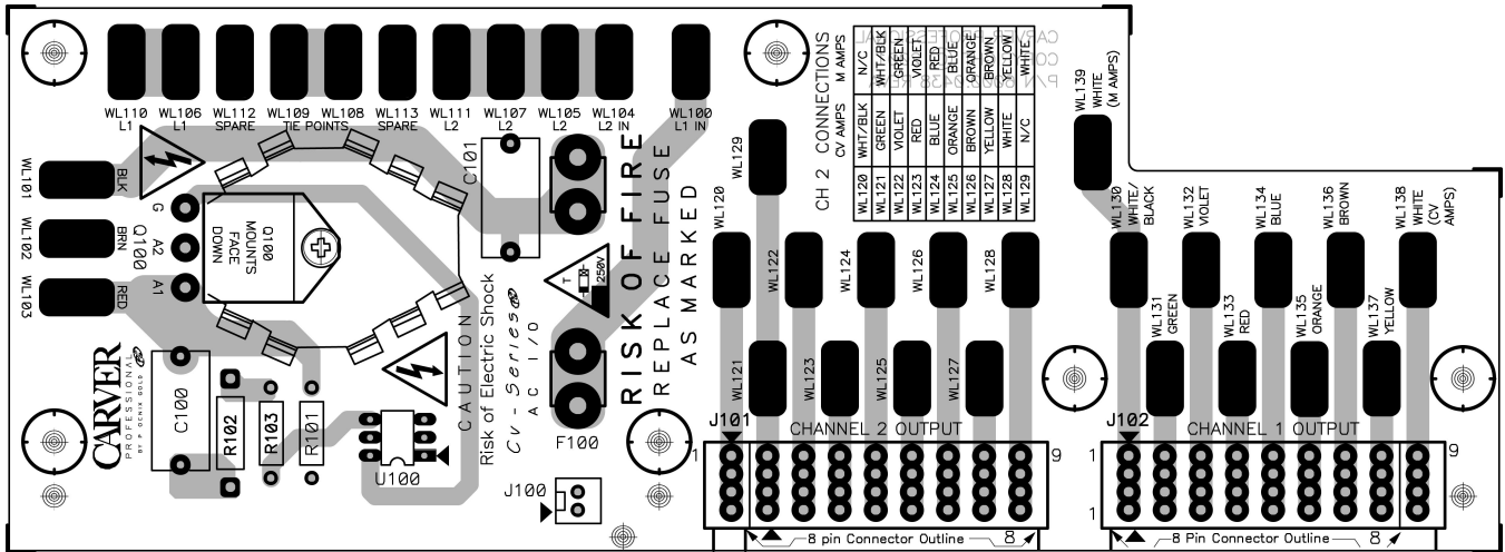
AC Input / Output PCB Bottom Etch Layout
