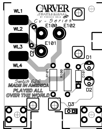
Switch PCB Bottom Etch Layout
