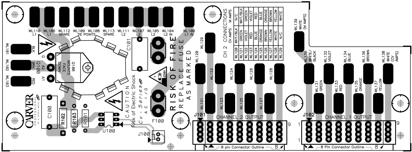
AC Input / Output PCB Top Etch Layout
