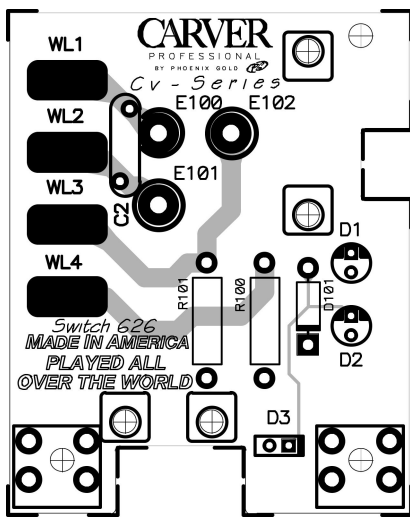
Switch PCB Top Etch Layout
