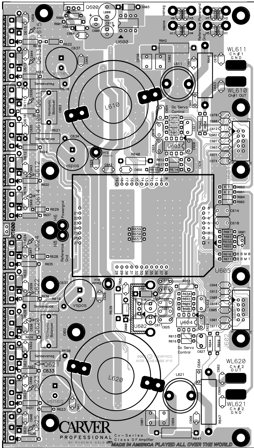
Amplifier PCB, Board Version 6000.0435 Bottom Etch Layout
