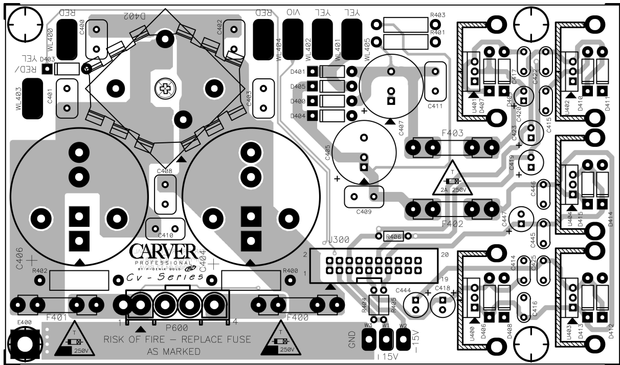
Power Supply PCB Bottom Etch Layout
