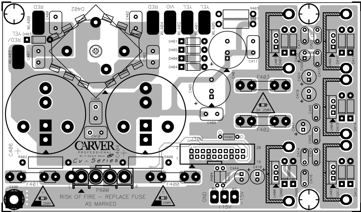
Power Supply PCB Top Etch Layout
