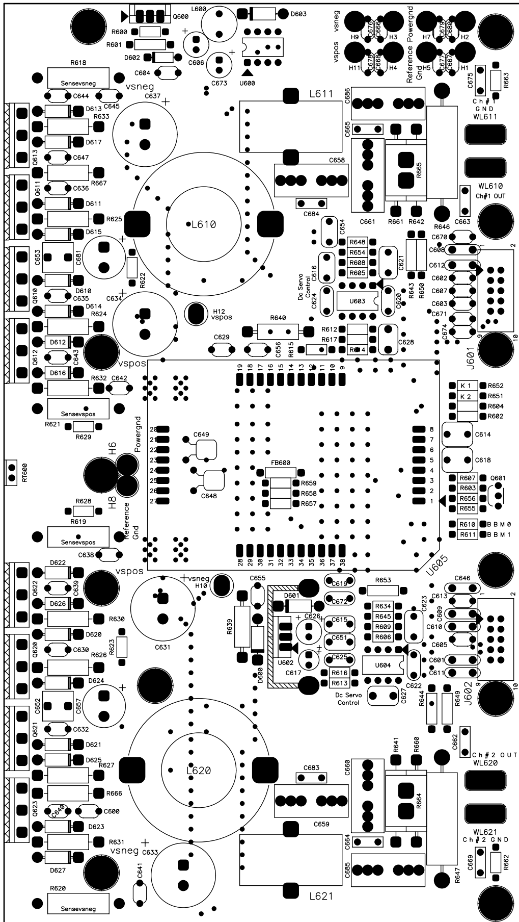
Amplifier PCB, Board Version 8005.0587 Top Component Layout
