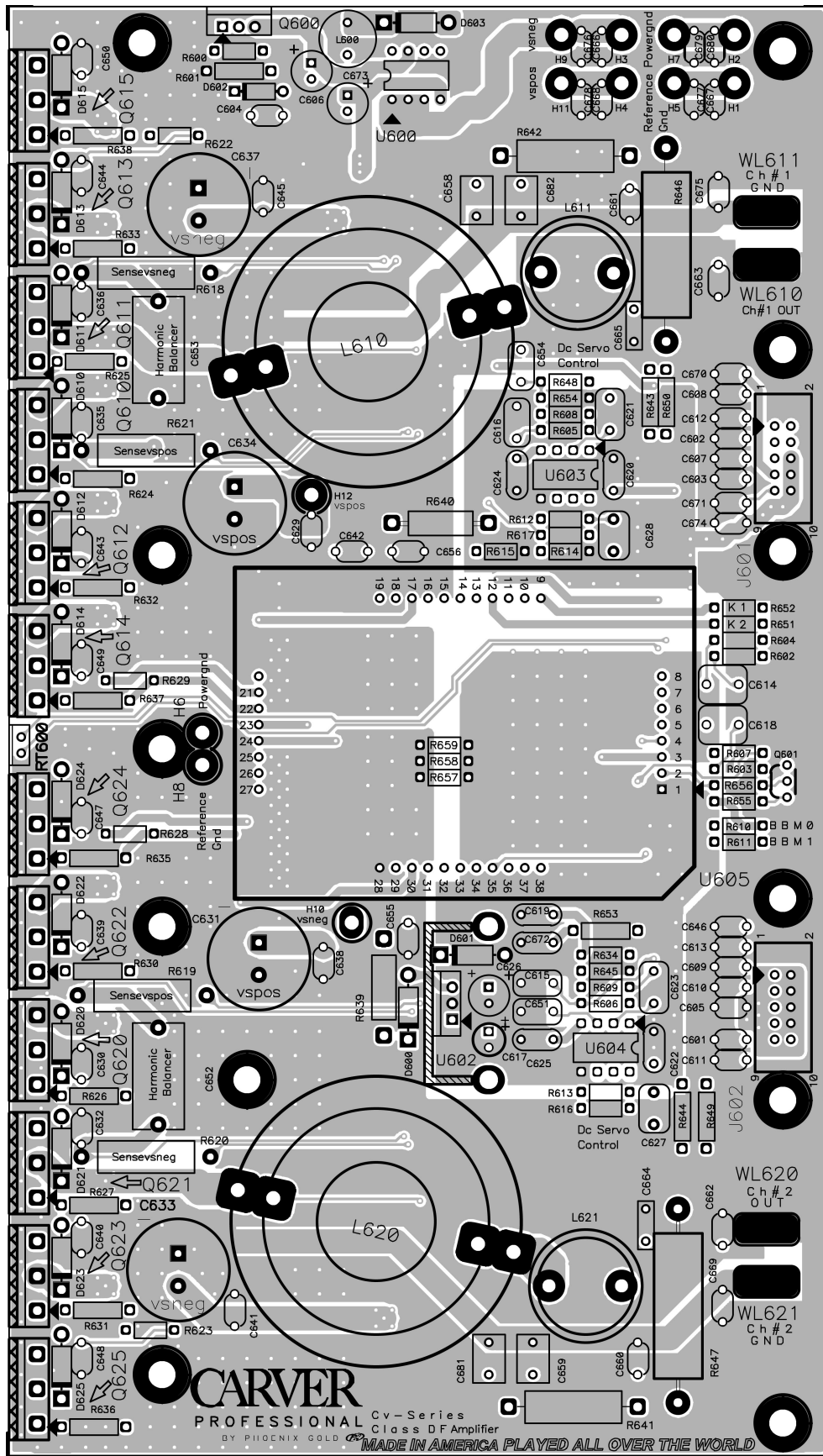
Amplifier PCB, Board Version 6000.0435 Top Etch Layout
