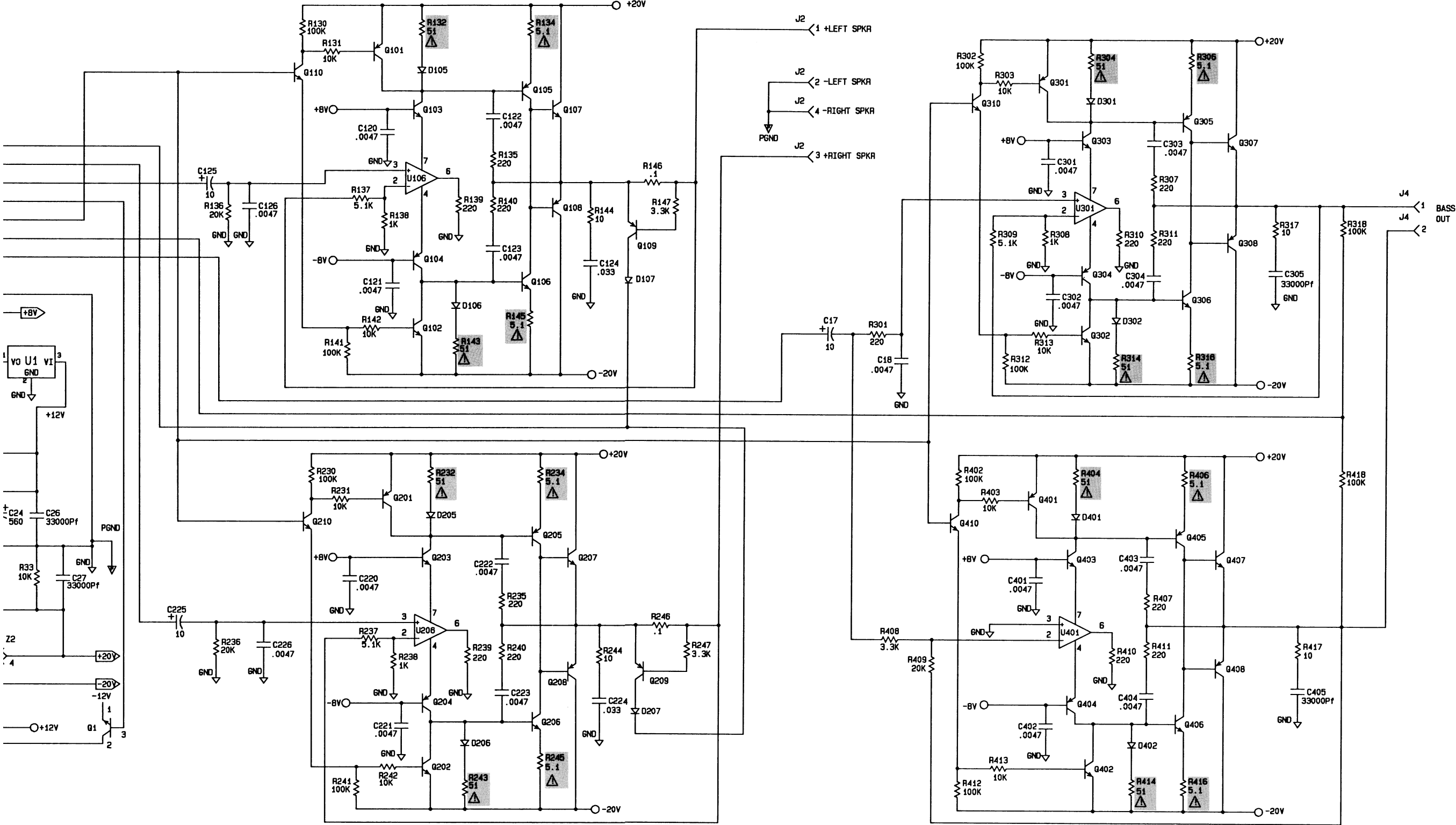
AM-3P Amplifier PCB Schematic
