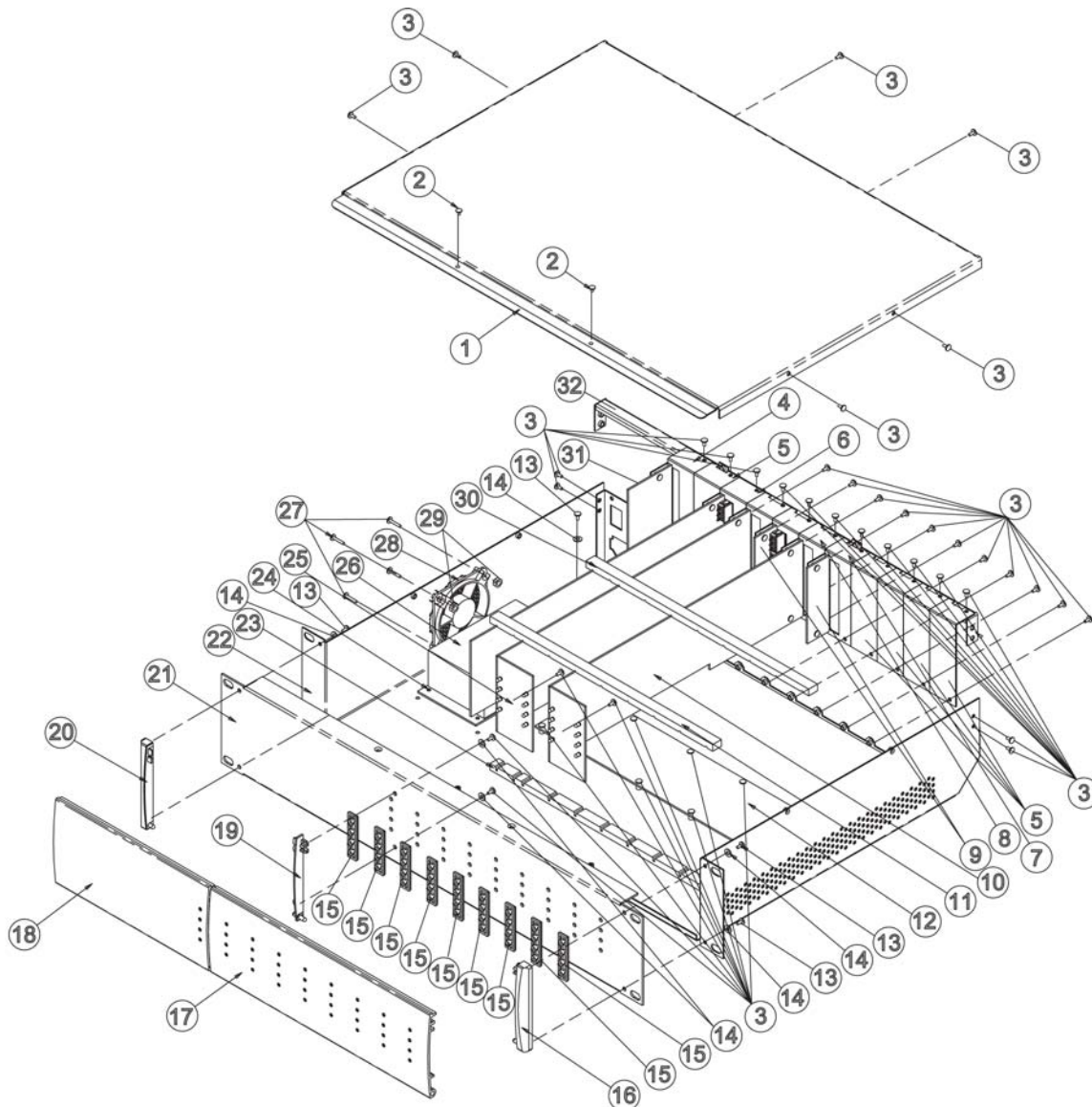
Figure 4. ControlSpace ESP-88C/ESP-00 Chassis Exploded View
