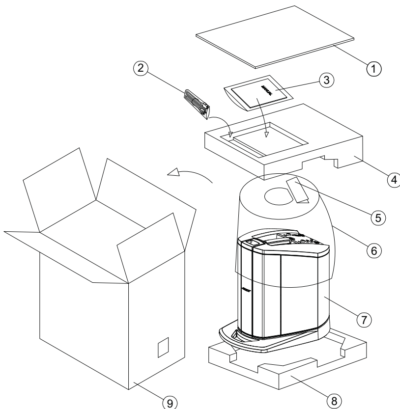
Figure 1. L1 Compact Power Stand Packaging View
