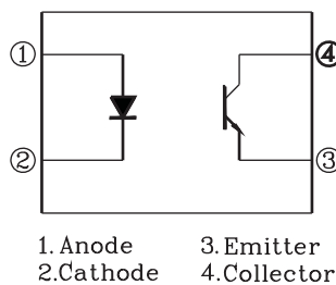
EL817 Photocoupler
