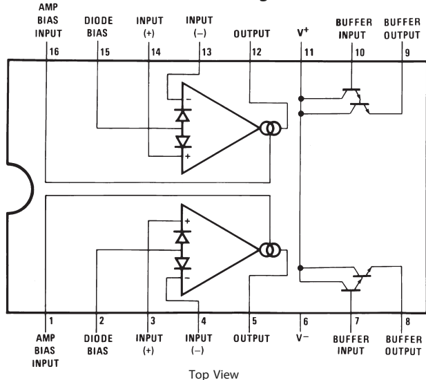
LM13700 Transconductance Amplifier
