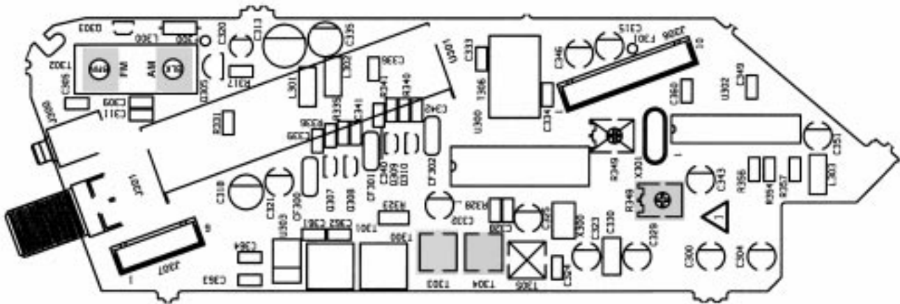
PCB 199827
