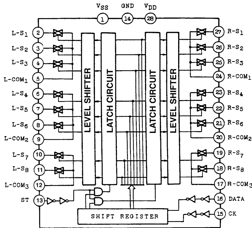
U101 Analog Switch TC9163N
