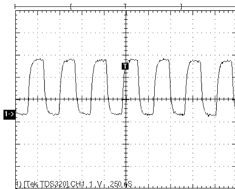
DSP PCB, U103 Pin 43, _64FS
