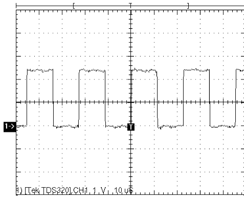
DSP PCB, U103 Pin 42, LRCLK
