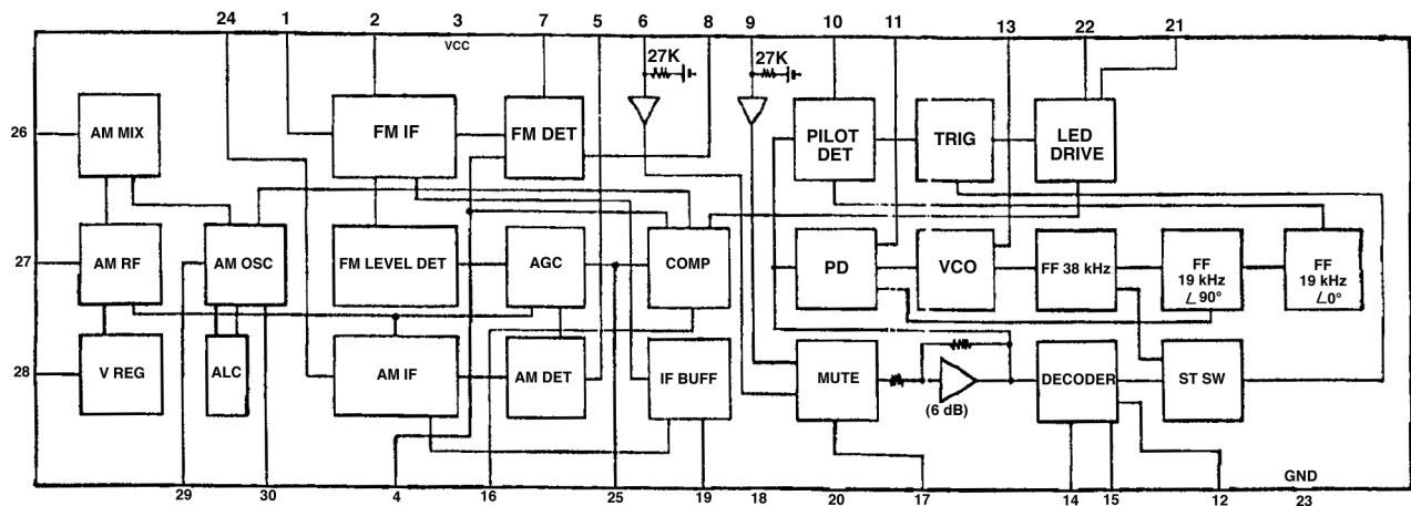
U301 AM/FM Tuner LA1851N
