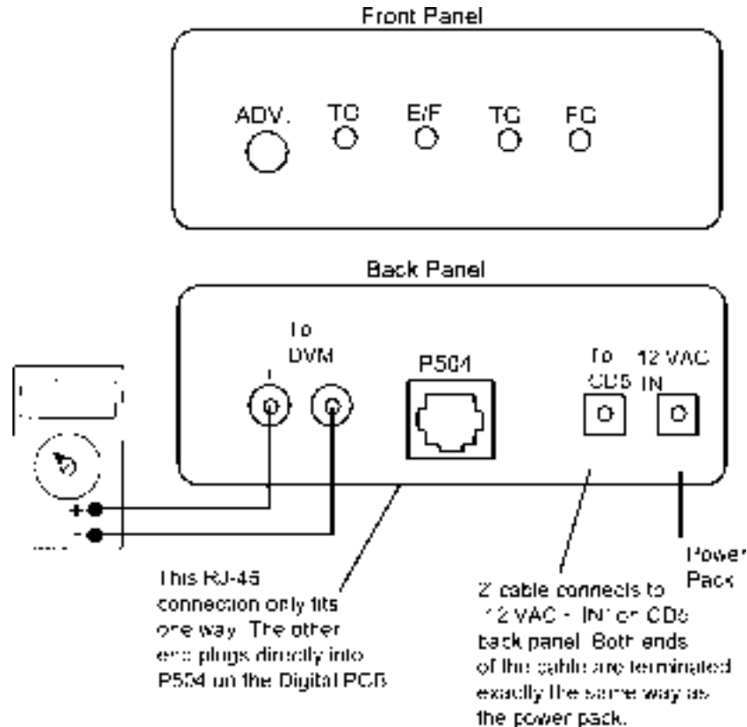
Figure 11. CD Alignment Fixture and Test Setup
