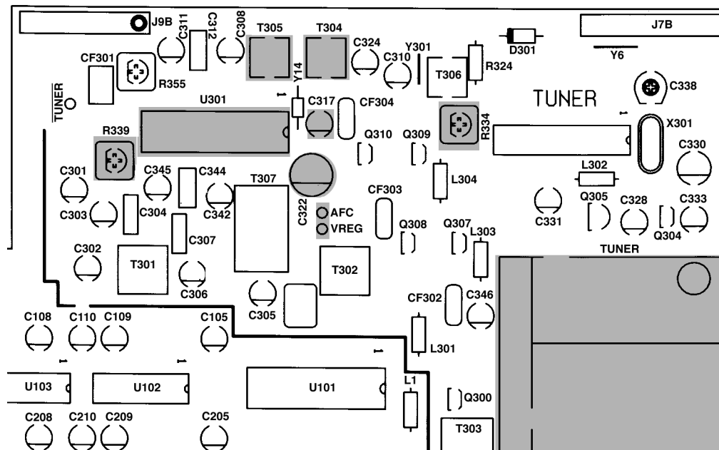
Figure 10. Audio PCB Test Section
