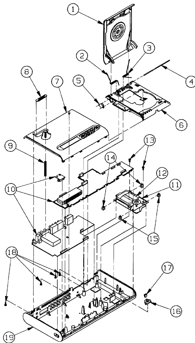
Figure 14. Exploded View
