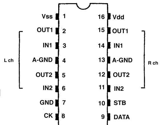
U103 Volume Control TC9213P
