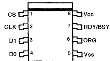
U401 EEPROM 59C11
