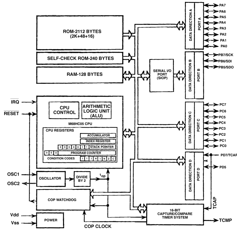
U505 Microcontroller 68HC05P7
