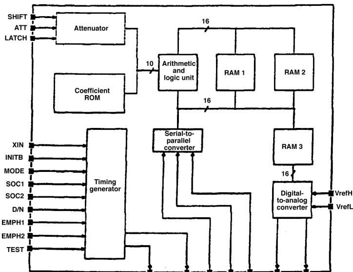
U506 D/A Converter
