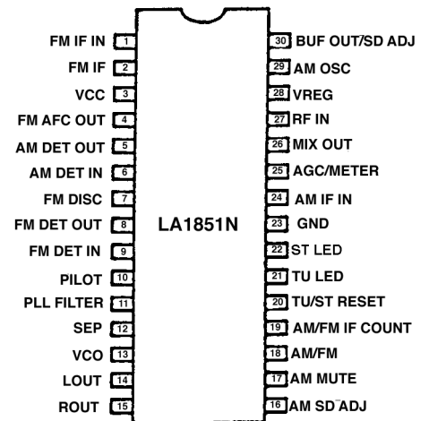
U301 AM/FM Tuner LA1851N
