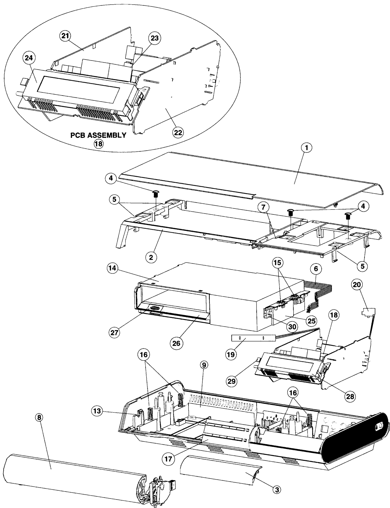
Figure 2. Disassembly/Assembly View
