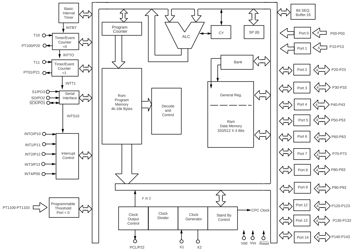
IC 601 (uPD75118GF-K12) Microprocessor
