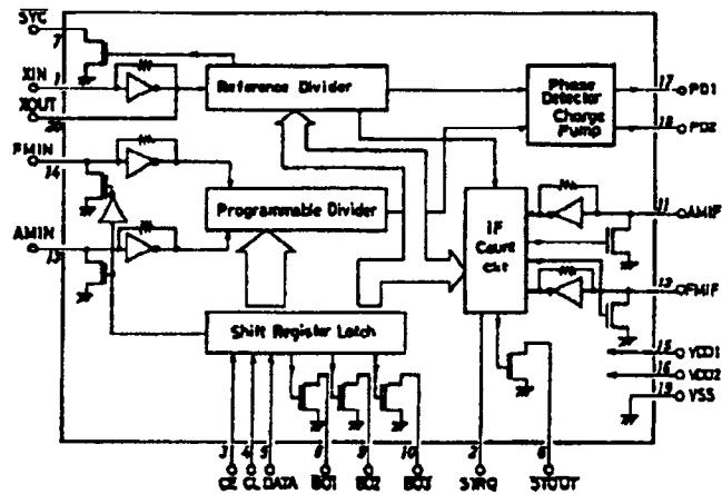
EQUIVALENT CIRCUIT BLOCK DIAGRAM
