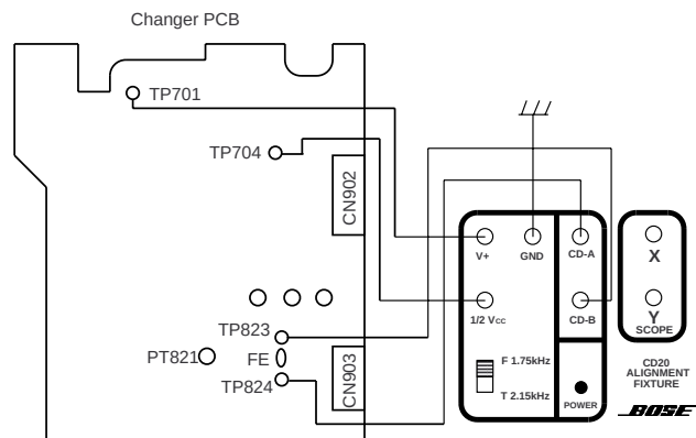
Figure 3. Focus Gain Alignment
