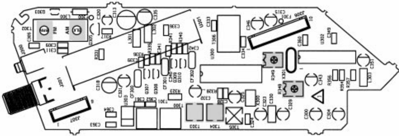
PCB 178335
