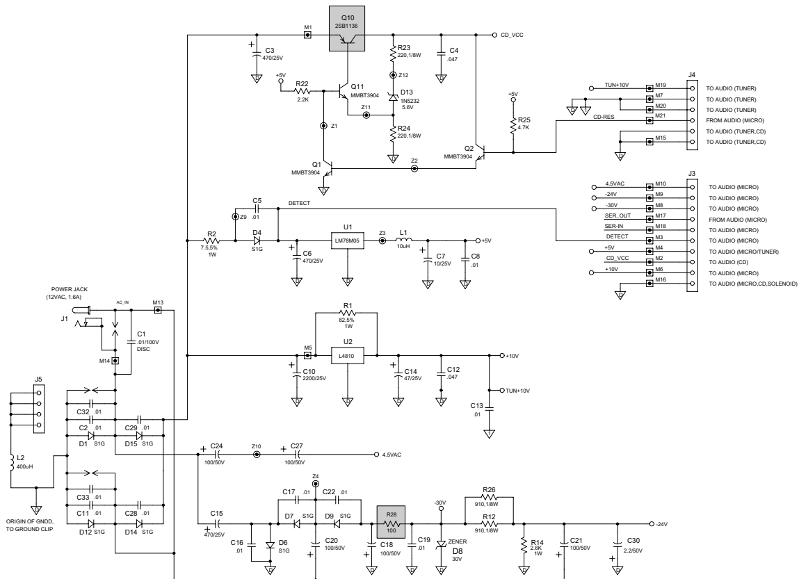
Power Supply Schematic Diagram PCB 250737
