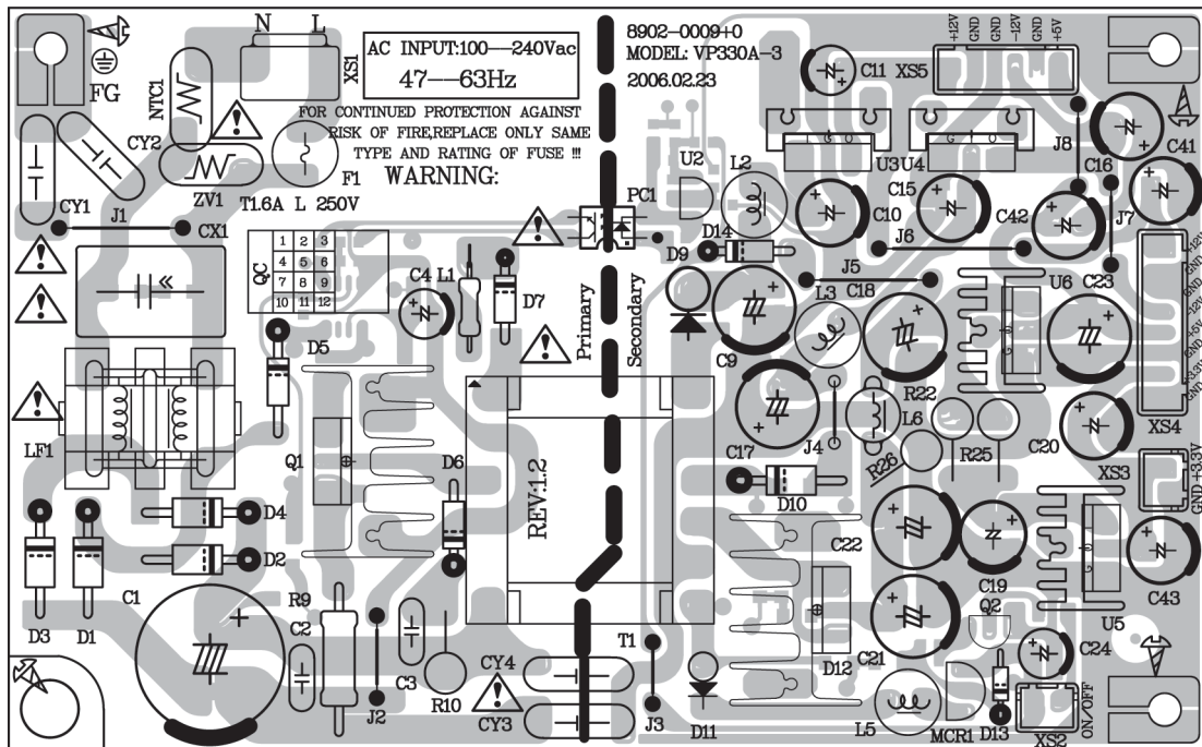
Figure 14. Switch Mode Power Supply PCB Top Etch and Component Layout
