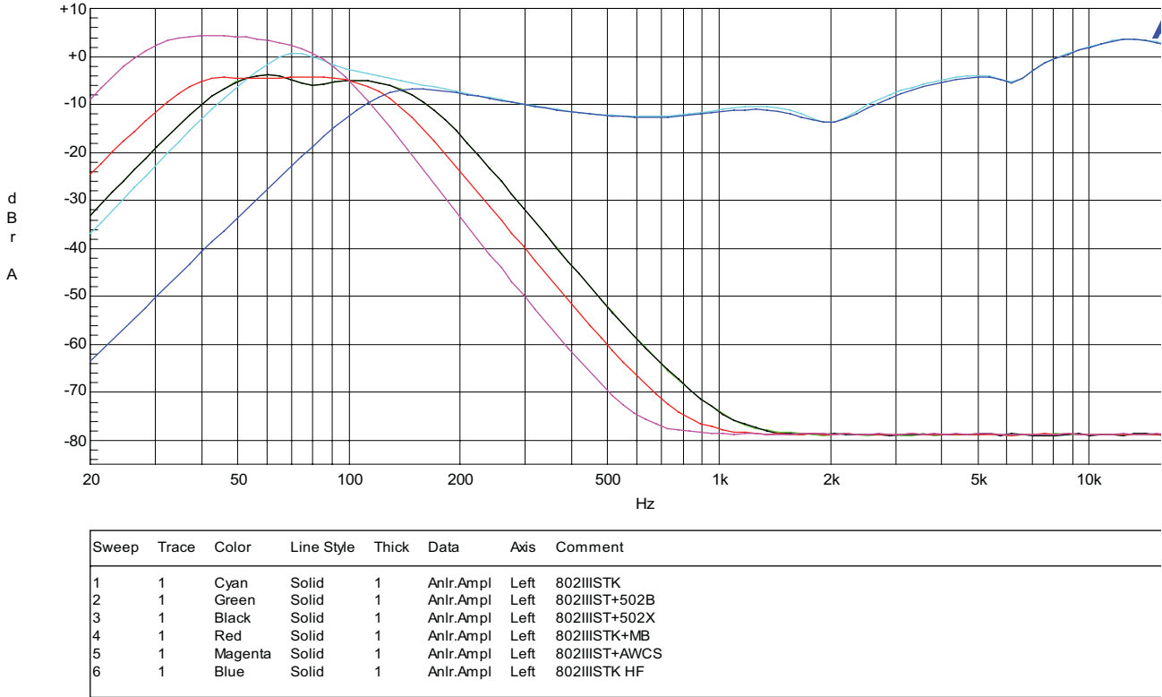
802IIIST CH3, 4
