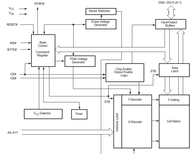
Block Diagram
