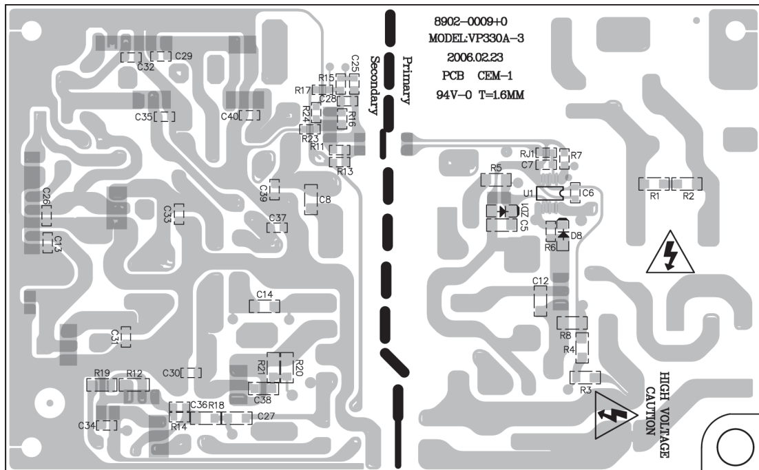
Figure 15. Switch Mode Power Supply PCB Bottom Etch and Component Layout
