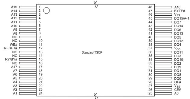
Pin Configuration
