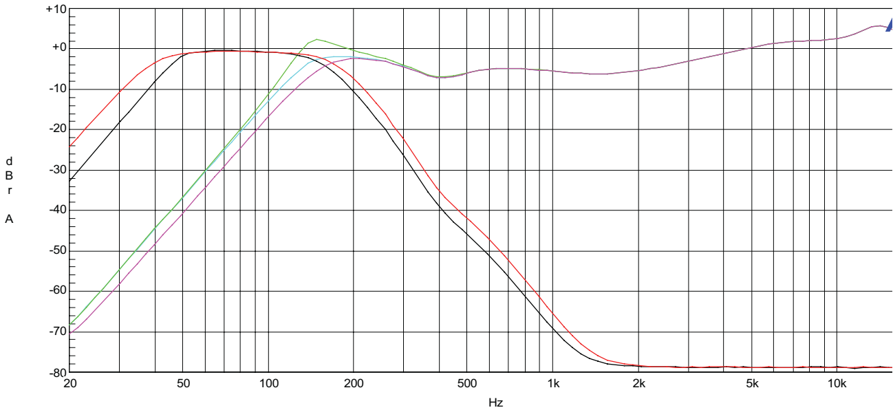
MA12STK CH1, 2
