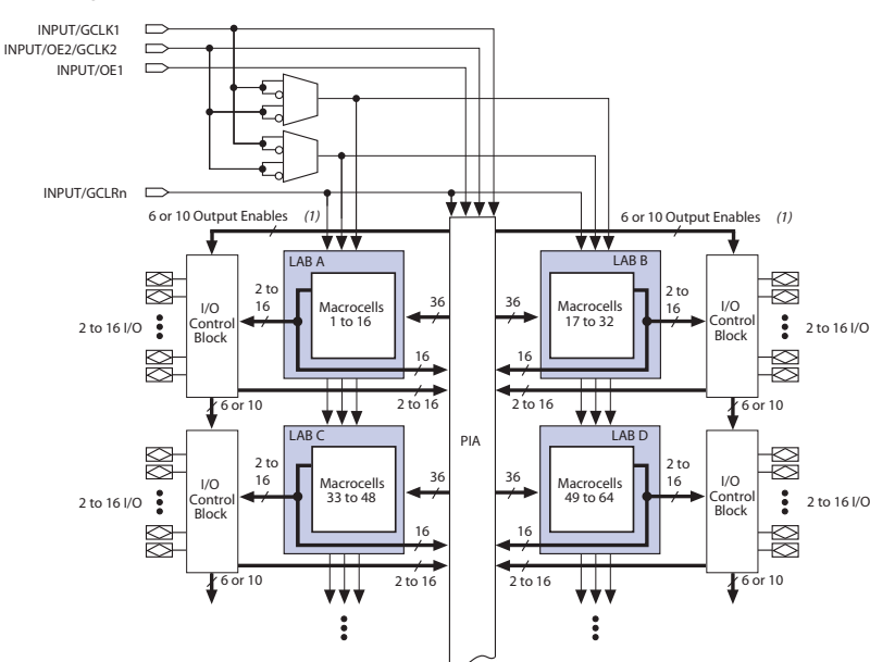
Block Diagram
