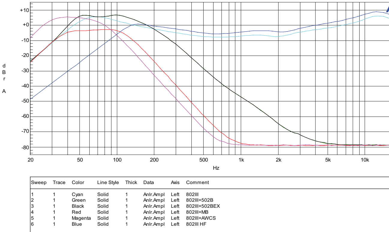
802III CH3, 4
