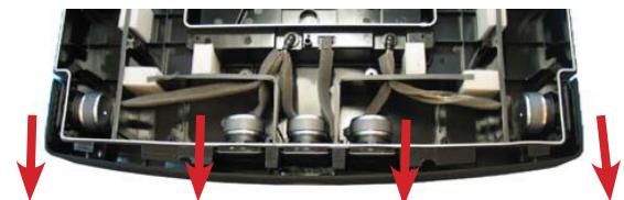
Figure 7B. Cloth Grille Removal
