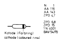
Dioden diodes
