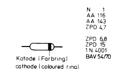
Dioden diodes
