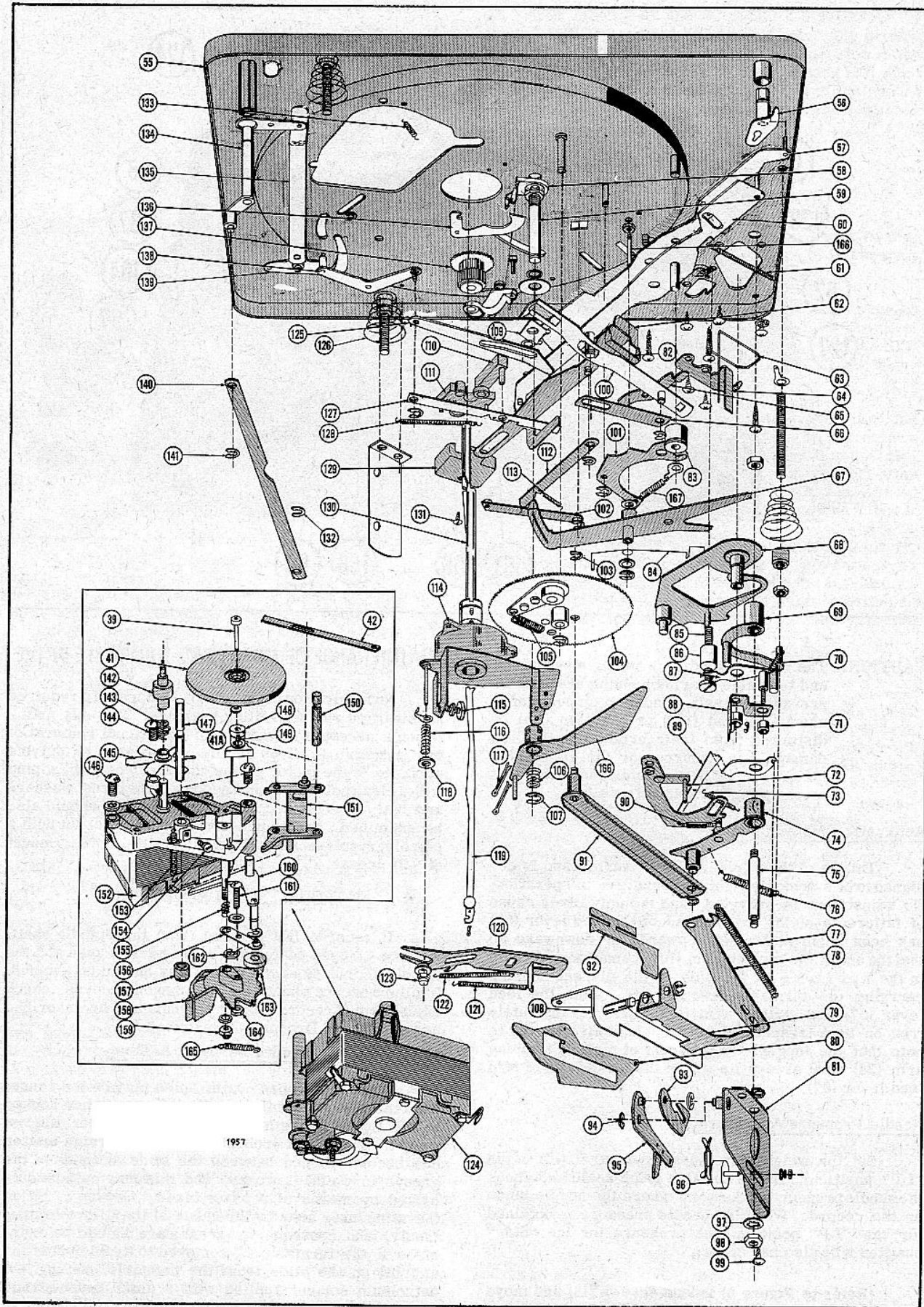
FIGURE 6B. EXPLODED VIEW OF PARTS BELOW BASEPLATE.
