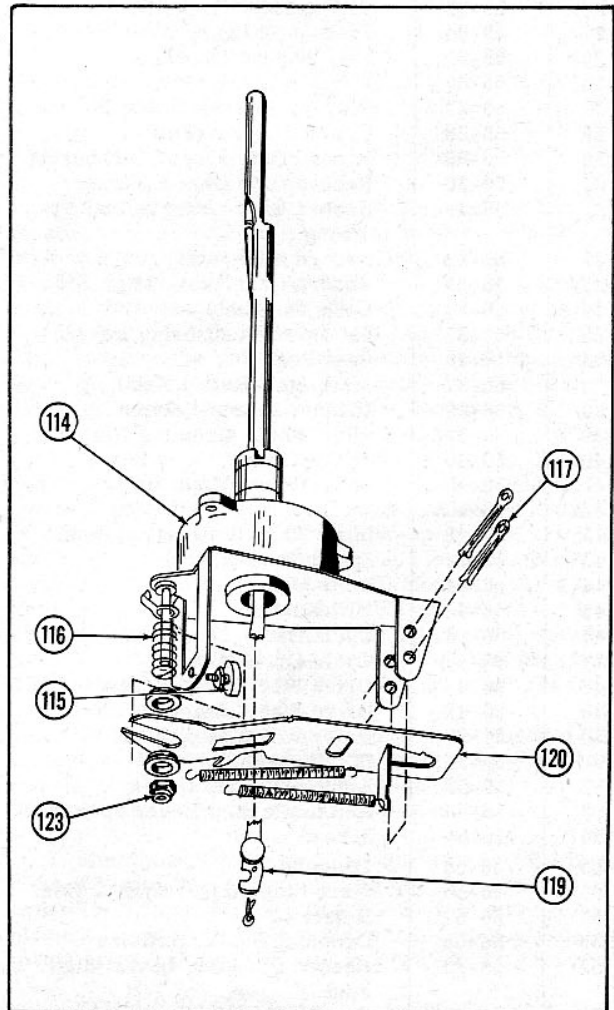
RECORD DROPPING MECHANISM
