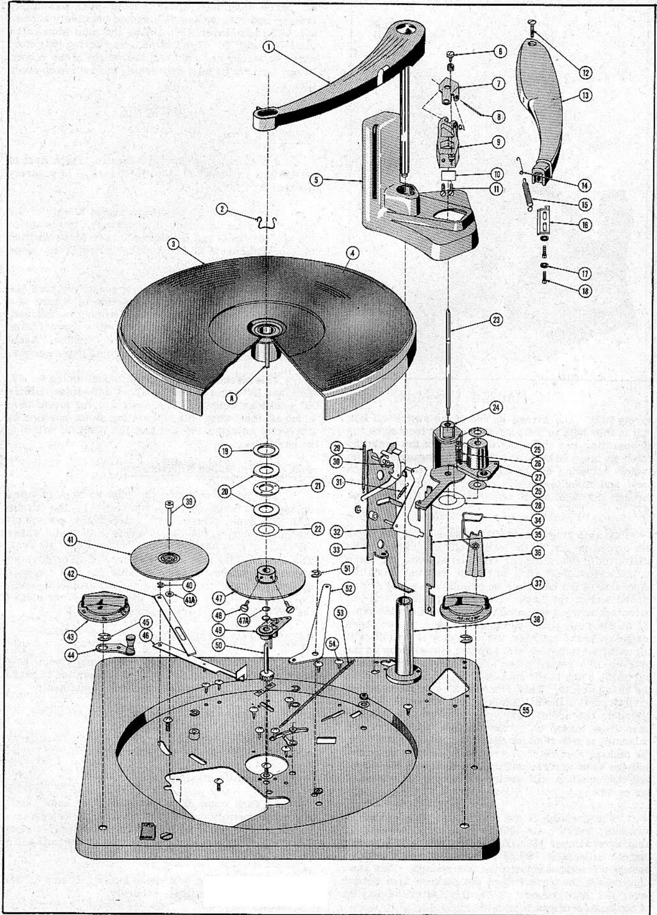
FIGURE 6A. EXPLODED VIEW OF PARTS ABOVE BASEPLATE.
