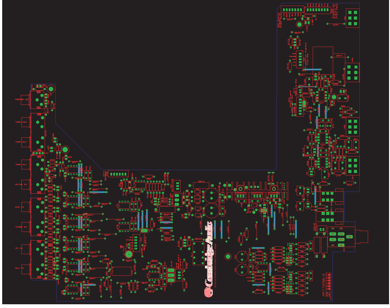
API 7649/4 Input PCB Board Layout (Top Side)
