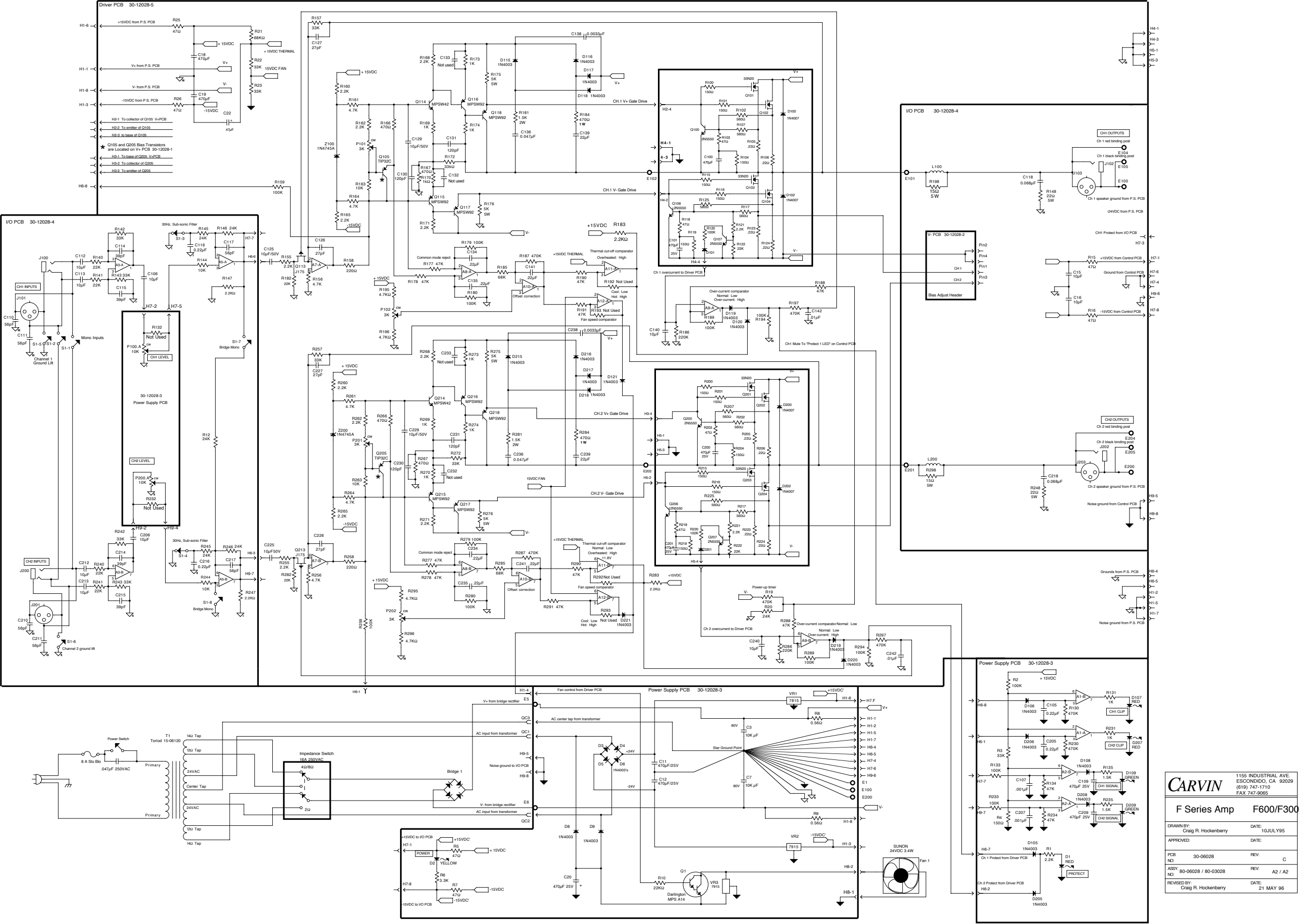
Driver PCB 30-12028-5
