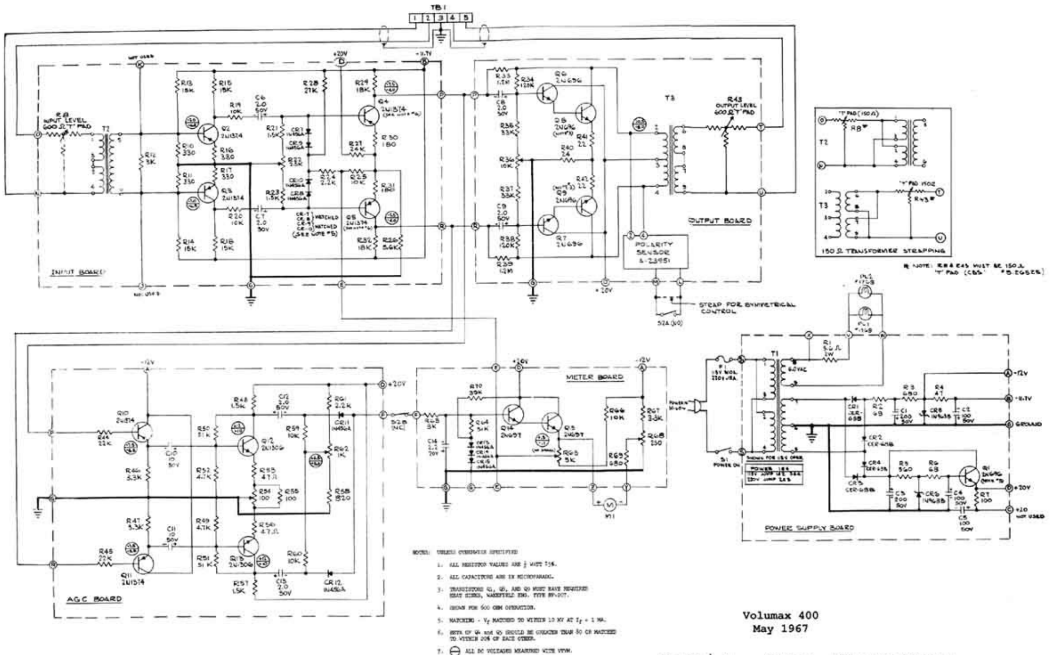
Figure 4-2. Volumax - Schematic Diagram
