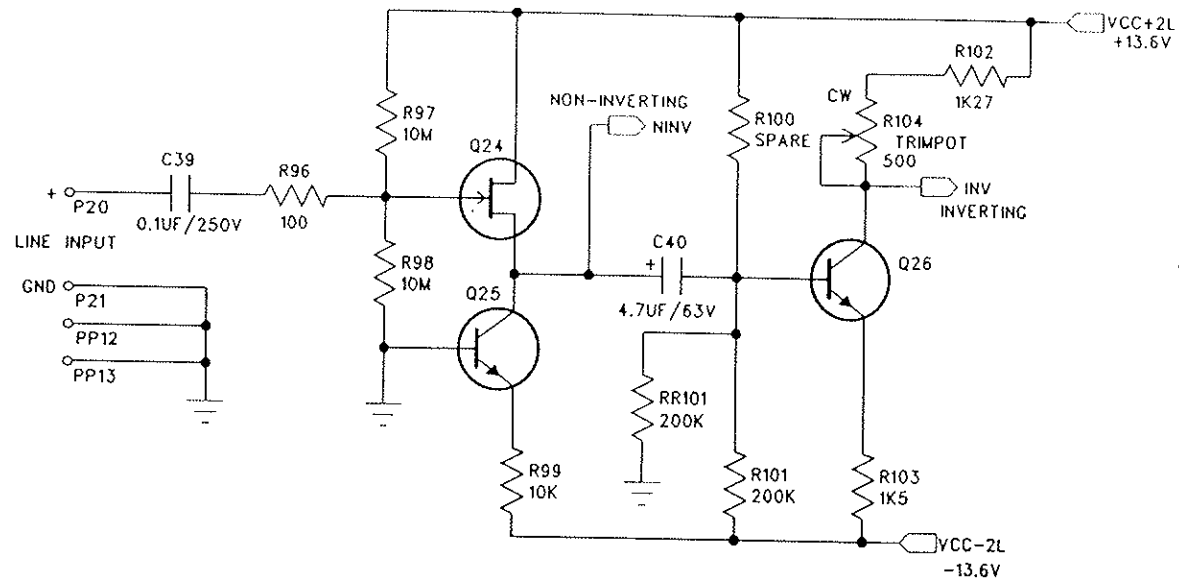
LINE BUFFER & INVERTER (LEFT CH.)
