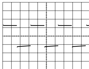
20 (IC501-76) 5Vp-p 2V/5μsec/cm REC/PLAY
