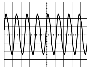
25 (IC501-38) 2.6Vp-p 0.5V/0.1μsec/cm REC/PLAY
