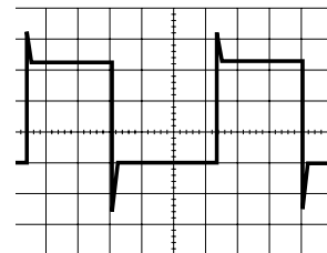
21 (IC501-94) 3Vp-p 1V/5msec/cm REC
