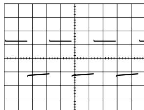
20 (IC501-76) 5Vp-p 2V/5µsec/cm REC/PLAY
