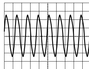
25 (IC501-38) 2.6Vp-p 0.5V/0.1µsec/cm REC/PLAY
