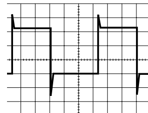
21 (IC501-94) 3Vp-p 1V/5msec/cm REC
