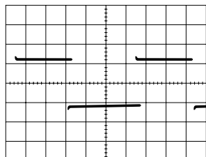
18 (IC501-18) 5Vp-p 2V/5msec/cm REC/PLAY
