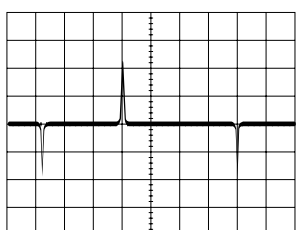
22 (IC501-97) 4.4Vp-p 1V/5msec/cm PLAY
