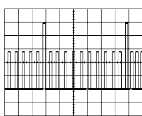
23 (IC501-90) 25Vp-p & 5Vp-p 1V/5msec/cm REC/PLAY
