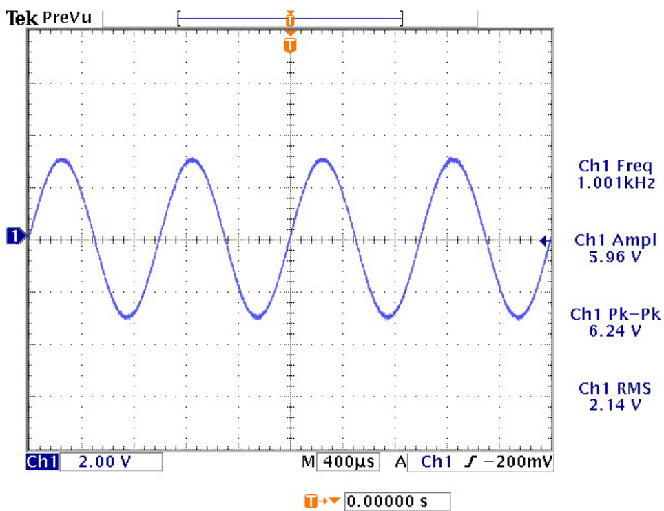
CP3 Pin 7&8(1KHz_AUDIO OUT)
