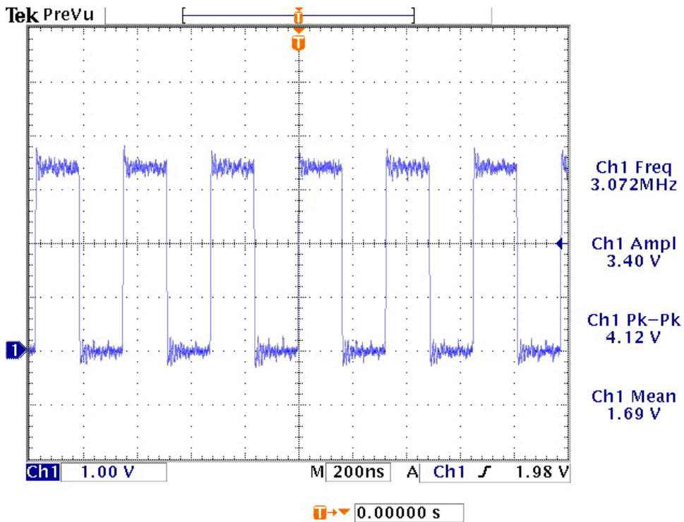
(AUDIO SBCLK) U16:CS4360 Pin5
