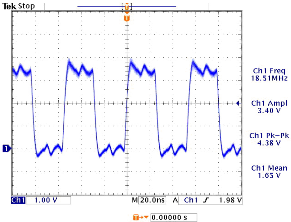
(AUDIO SACLK) U16:CS4360 Pin7
