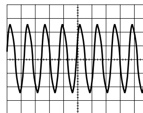
25 (IC501-38) 2.6Vp-p 0.5V/0.1μsec/cm REC/PLAY
