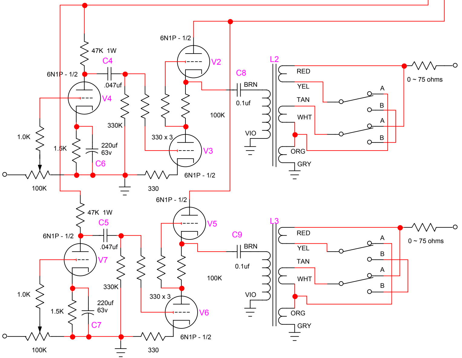
DECWARE TUBE HEADPHONE AMPLIFIER MODEL MLB ~ "My little budy" drives headphones from 30 ~ 600 ohms
