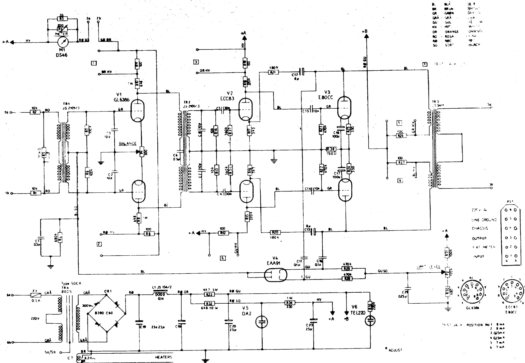
DISA Limiting Amplifier Type 91N02
