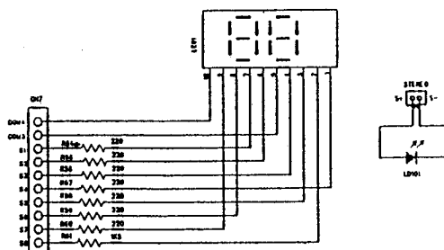
DISPLAY BOARD
