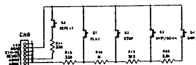
KEY BOARD
