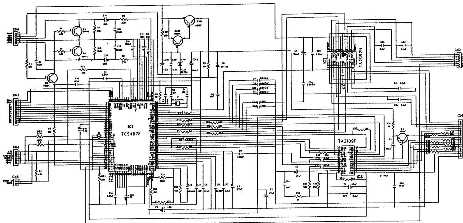
CD BOARD
