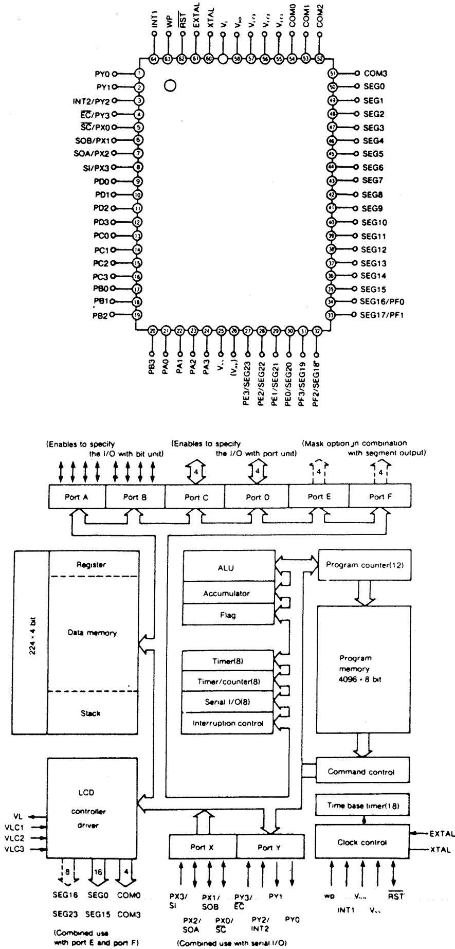
Pin Configuration Diagram(Top View)
