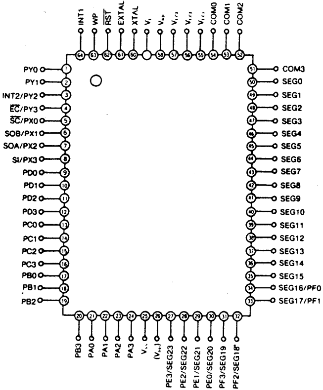
Pin Configuration Diagram(Top View)
