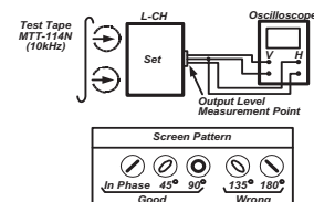
FIG. 4 : Tape Azimuth Adjust Circuit & Waveform
