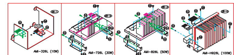
AMI-326L/726L/826L/H926L EXPLODED VIEW
