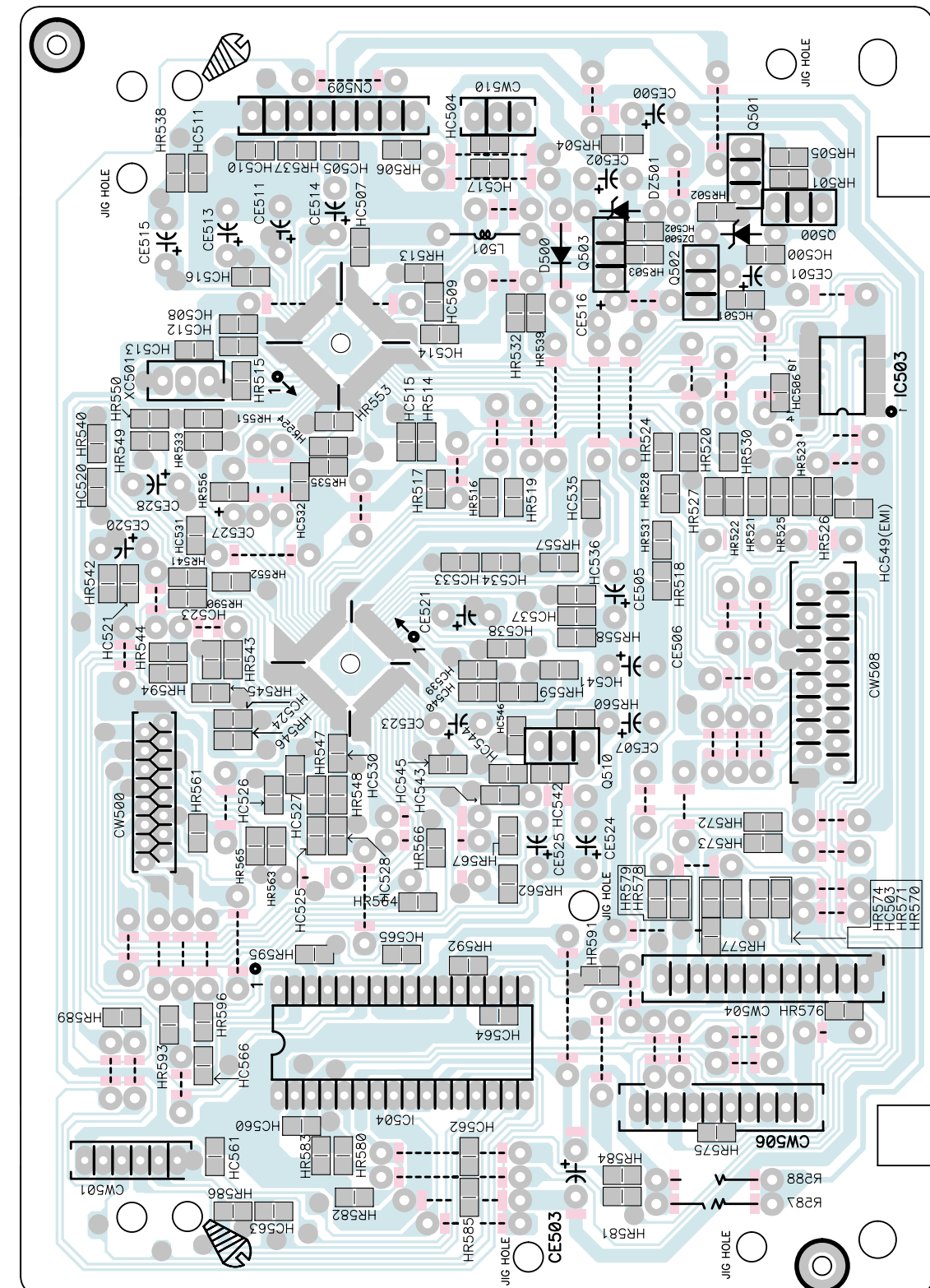
<BOTTOM VIEW>
