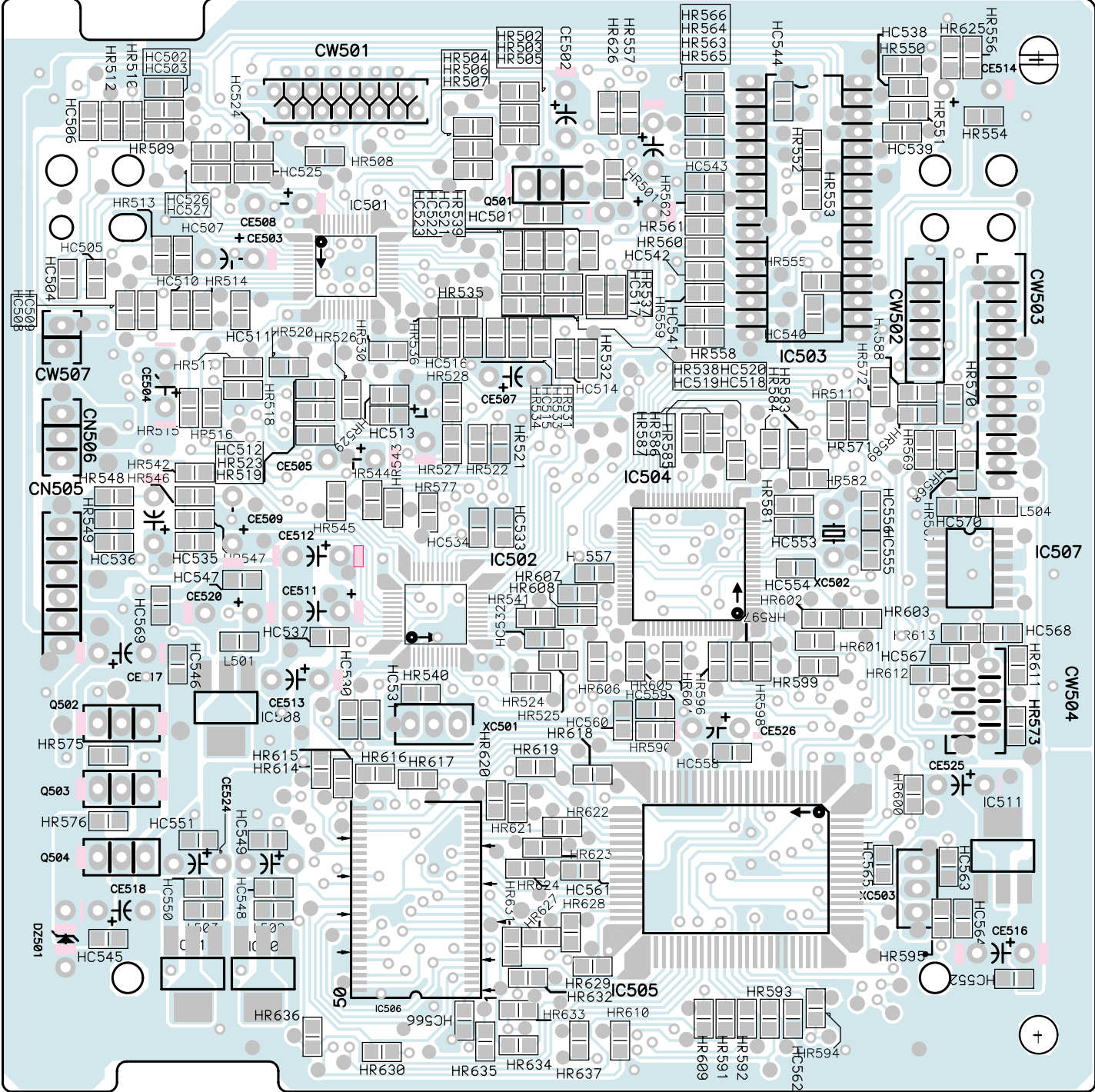
<BOTTOM VIEW>
