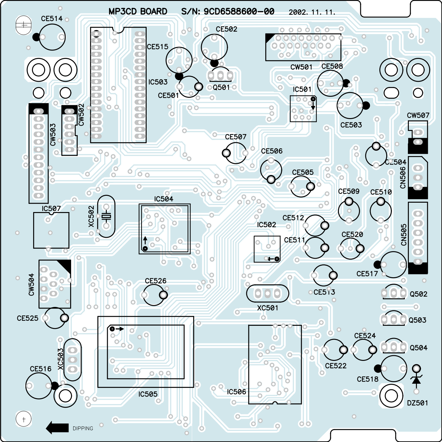
<TOP VIEW>
