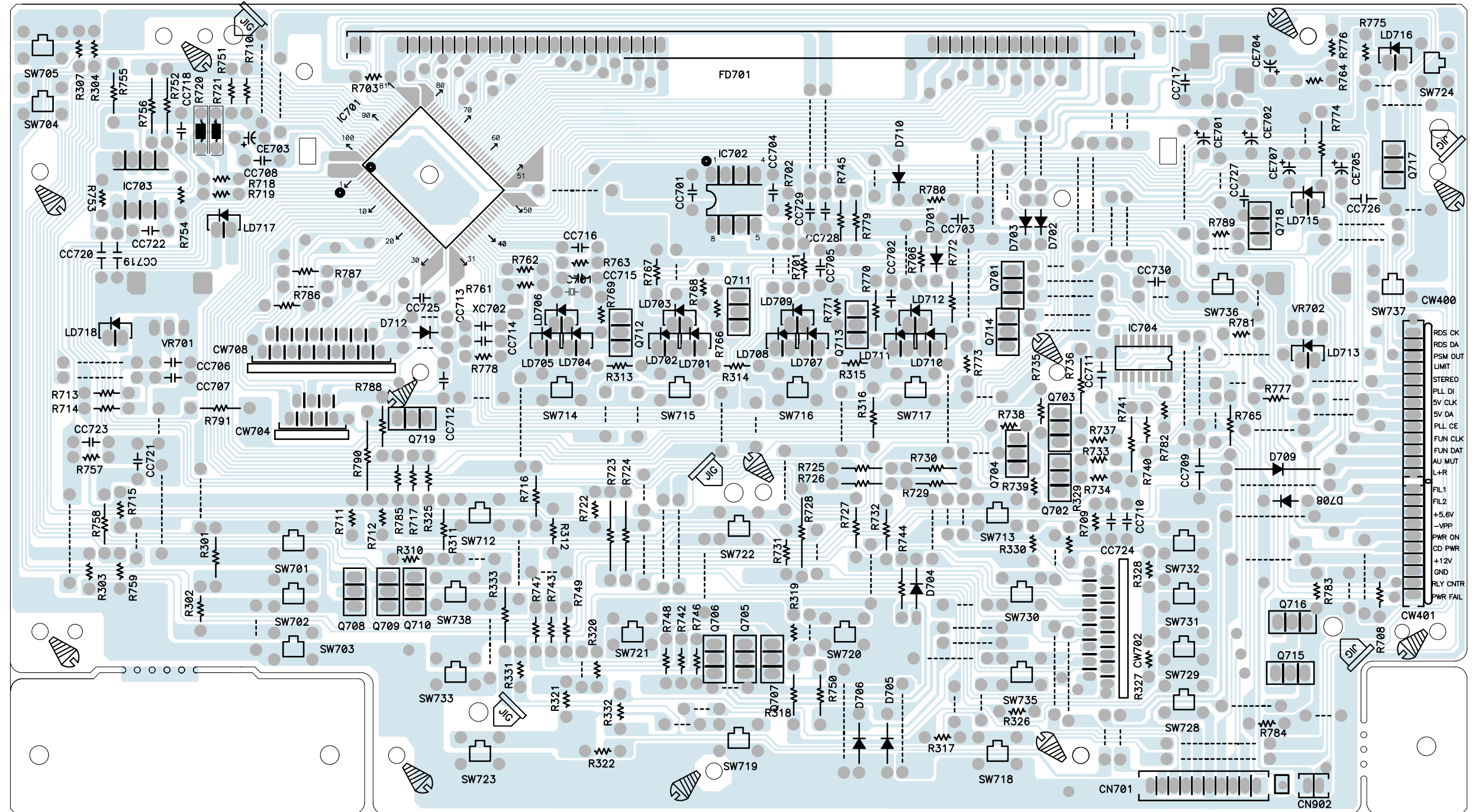
<BOTTOM VIEW>
