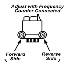
FIG. 2 : Tape Azimuth Adjust Location (Record/Playback Head)
