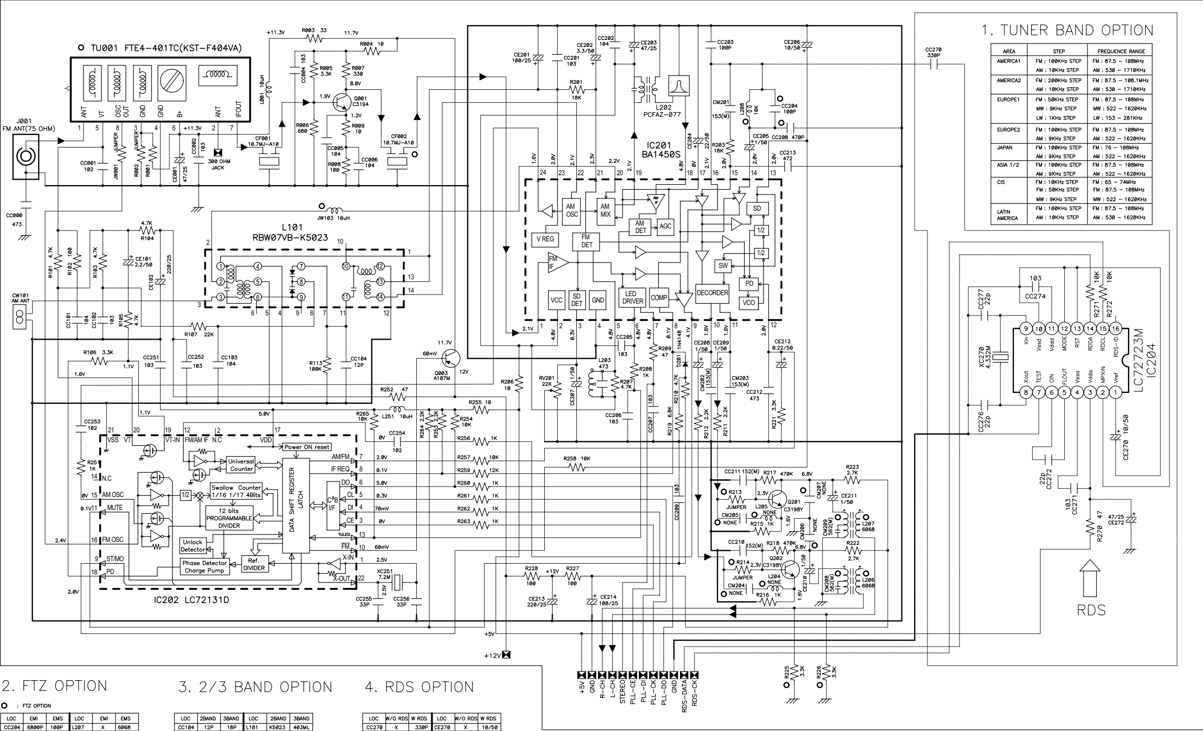
150W RW TUNER SCHEMATIC DIAGRAM(2BAND)
