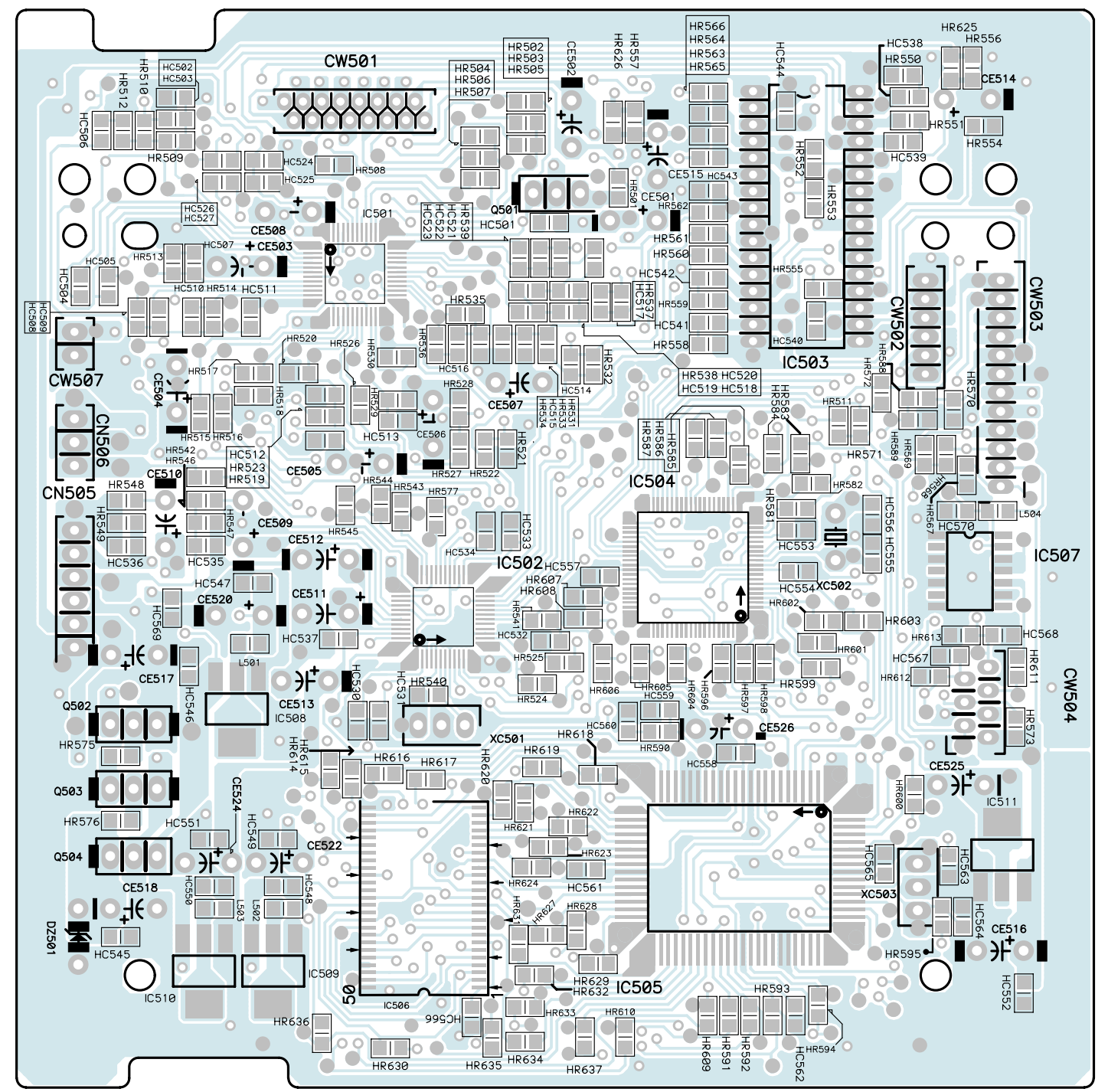
<BOTTOM VIEW>
