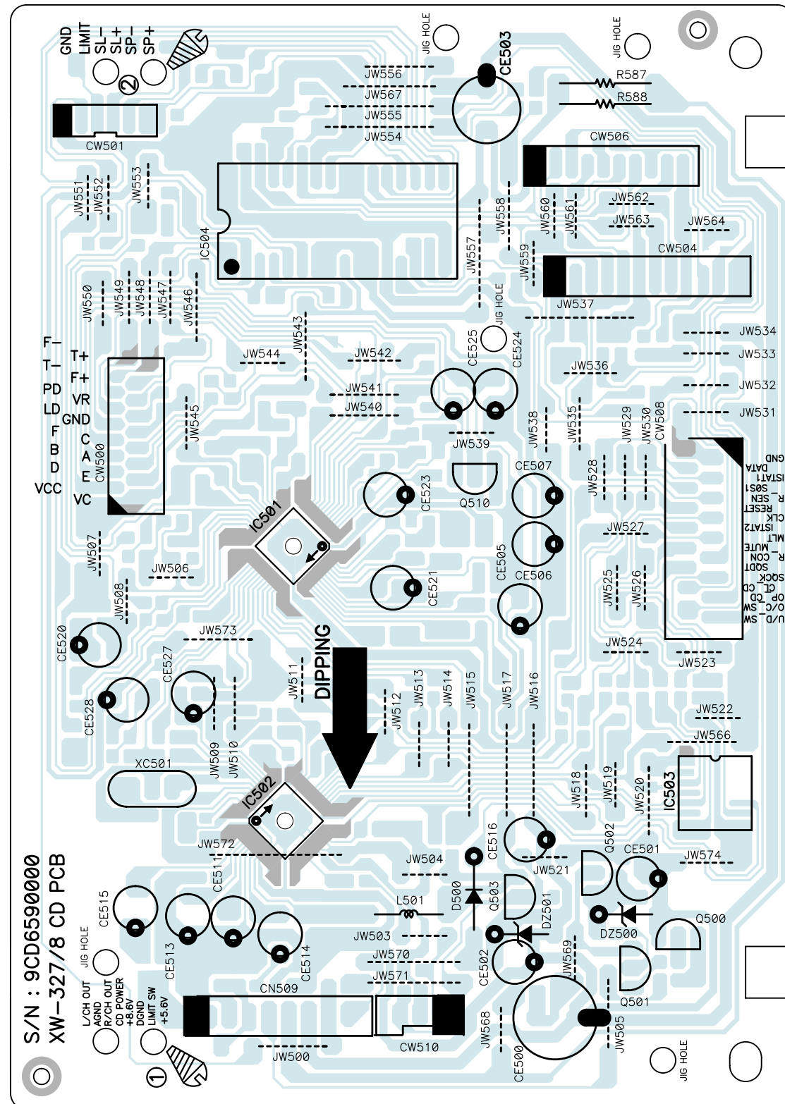
<TOP VIEW>
