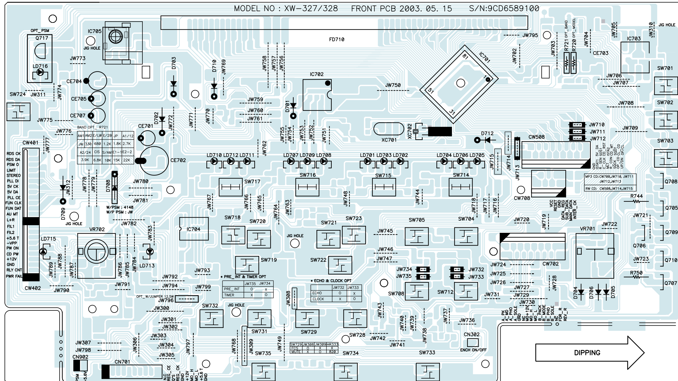
<TOP VIEW>
