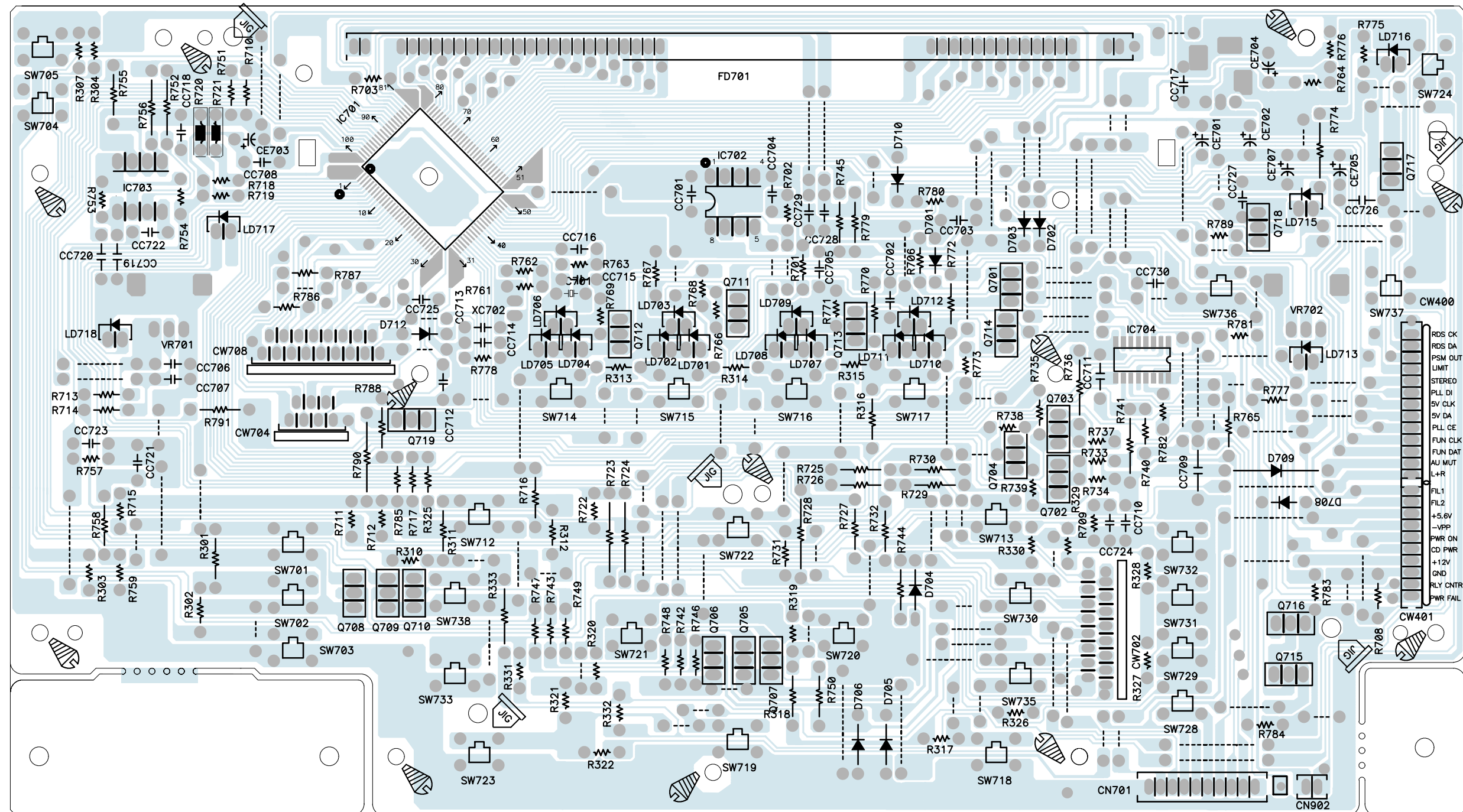
<BOTTOM VIEW>
