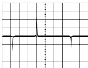
㉒ (IC501-97) 4.4Vp-p 1V/5msec/cm PLAY
