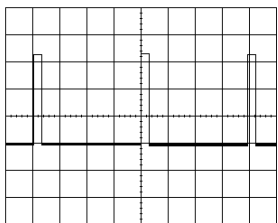
⑤ (IC301-67) 4.6Vp-p 2V/10usec/cm REC/PLAY
