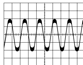
⑪ (IC301-8) 120mVp-p 50mV/0.5msec/cm PLAY
