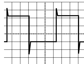
㉑ (IC501-94) 3Vp-p 1V/5msec/cm REC
