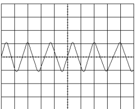
⑦ (IC301-28) 450mVp-p 200mV/0.1usec/cm
