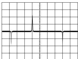
㉒ (IC501-97) 4.4Vp-p 1V/5msec/cm PLAY
