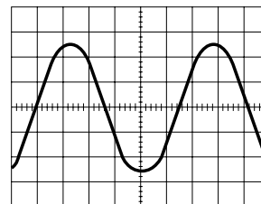
⑯ (IC251-32) 200mVp-p 50mV/0.5msec EE/REC
