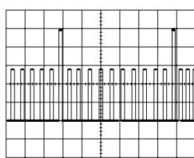
㉓ (IC501-90) 25Vp-p & 5Vp-p 1V/5msec/cm REC/PLAY
