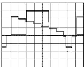
③ (IC301-43) 520mVp-p 100mV/5usec REC
