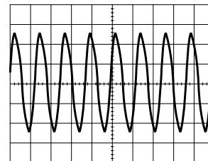
㉕ (IC501-38) 2.6Vp-p 0.5V/0.1μsec/cm REC/PLAY
