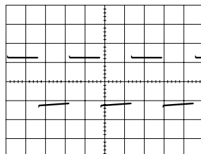
⑳ (IC501-76) 5Vp-p 2V/5μsec/cm REC/PLAY
