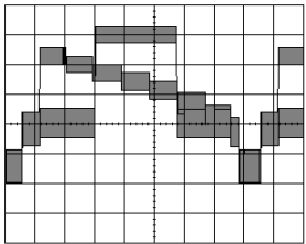
③ (IC301-43) 520mVp-p 100mV/5usec PLAY
