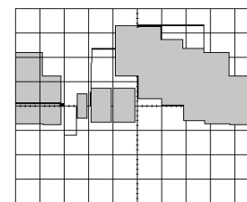
⑥ (IC301-65) 2.2Vp-p 500mV/5usec/cm PLAY
